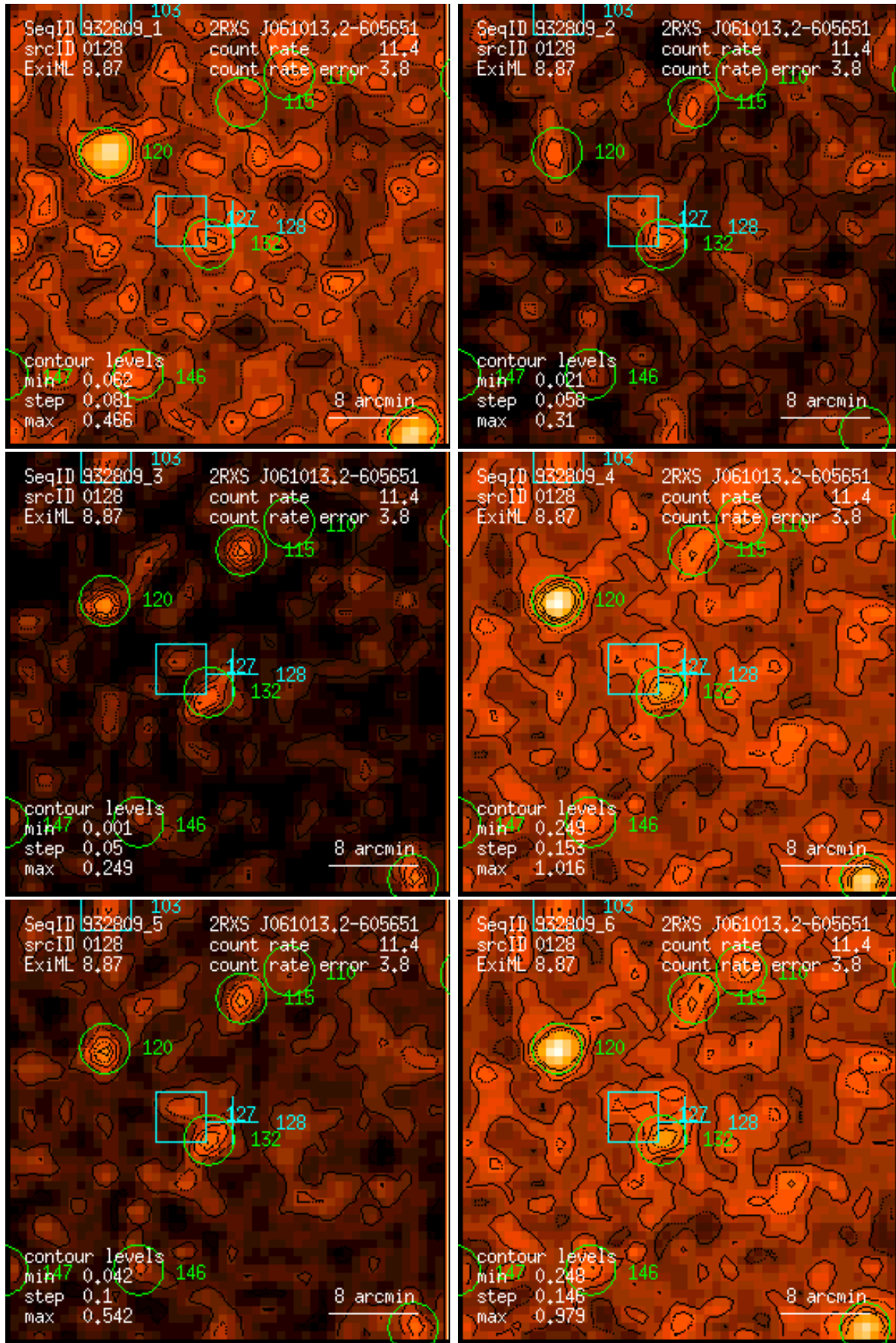
Figure 128: RASS 932809: detection 0128: band rate images, Gaussian filter: (1) PSPC channels 11 – 41, (2) 52 – 90, (3) 91 – 201, (4) 11 – 235, (5) 52 – 201, (6) 11 – 201. Broad band rates in counts/ks. Band rate contour levels in counts/ks/arcmin 2 .
