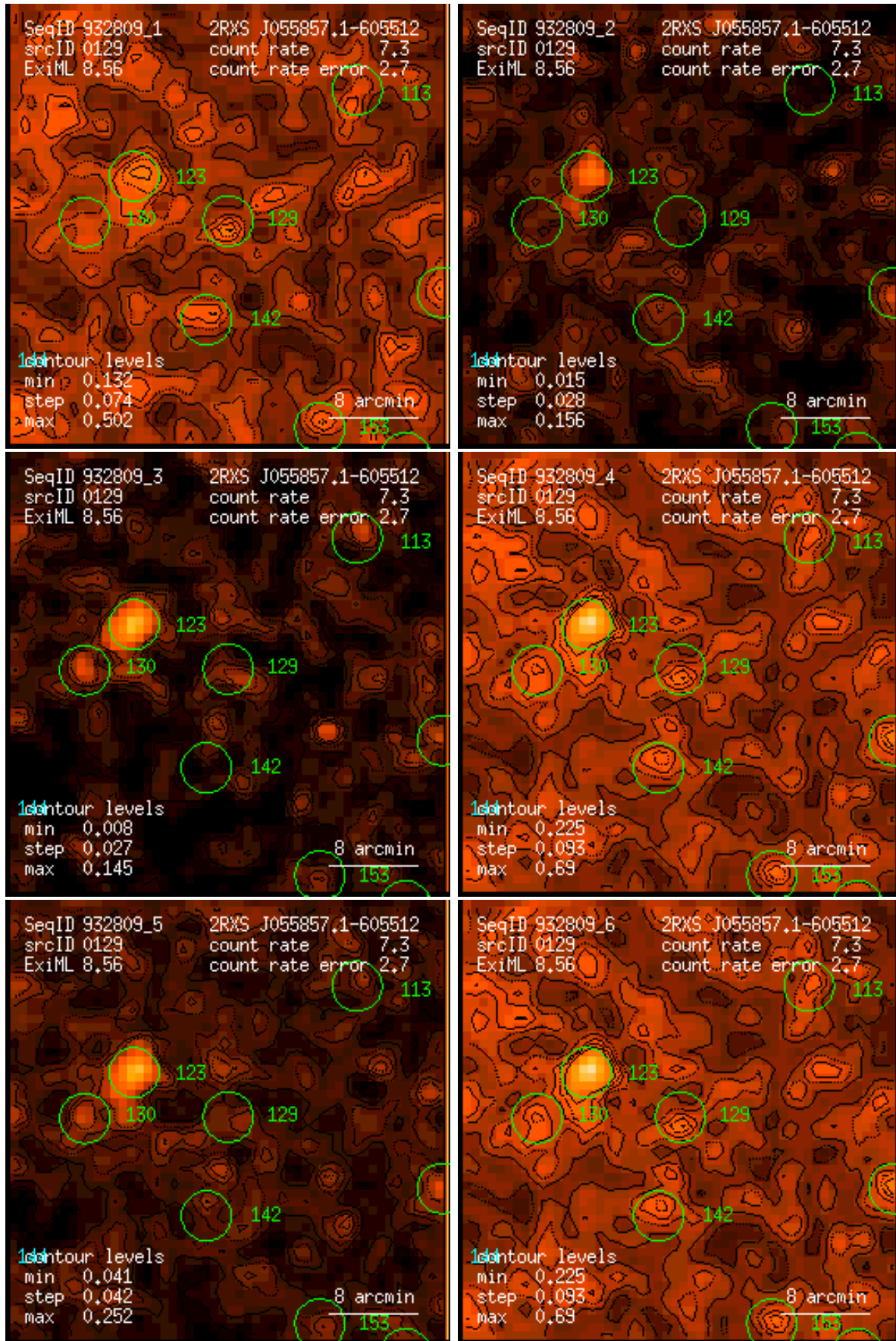
Figure 129: RASS 932809: detection 0129: band rate images, Gaussian filter: (1) PSPC channels 11 – 41, (2) 52 – 90, (3) 91 – 201, (4) 11 – 235, (5) 52 – 201, (6) 11 – 201. Broad band rates in counts/ks. Band rate contour levels in counts/ks/arcmin 2 .
