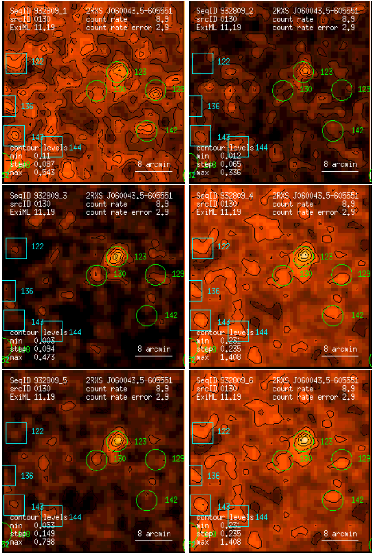
Figure 130: RASS 932809: detection 0130: band rate images, Gaussian filter: (1) PSPC channels 11 – 41, (2) 52 – 90, (3) 91 – 201, (4) 11 – 235, (5) 52 – 201, (6) 11 – 201. Broad band rates in counts/ks. Band rate contour levels in counts/ks/arcmin 2 .
