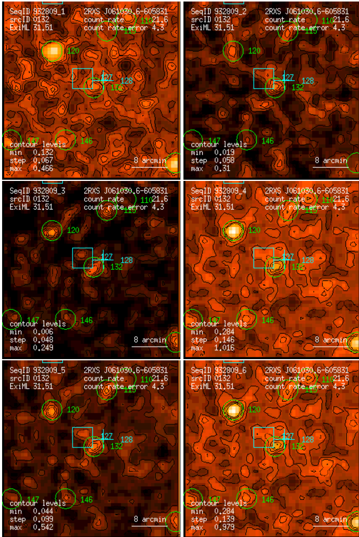
Figure 132: RASS 932809: detection 0132: band rate images, Gaussian filter: (1) PSPC channels 11 – 41, (2) 52 – 90, (3) 91 – 201, (4) 11 – 235, (5) 52 – 201, (6) 11 – 201. Broad band rates in counts/ks. Band rate contour levels in counts/ks/arcmin 2 .
