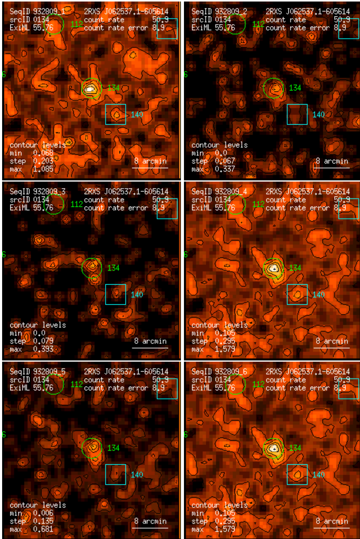
Figure 134: RASS 932809: detection 0134: band rate images, Gaussian filter: (1) PSPC channels 11 – 41, (2) 52 – 90, (3) 91 – 201, (4) 11 – 235, (5) 52 – 201, (6) 11 – 201. Broad band rates in counts/ks. Band rate contour levels in counts/ks/arcmin 2 .
