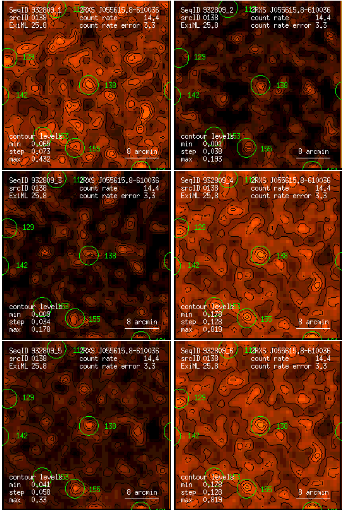
Figure 138: RASS 932809: detection 0138: band rate images, Gaussian filter: (1) PSPC channels 11 – 41, (2) 52 – 90, (3) 91 – 201, (4) 11 – 235, (5) 52 – 201, (6) 11 – 201. Broad band rates in counts/ks. Band rate contour levels in counts/ks/arcmin 2 .
