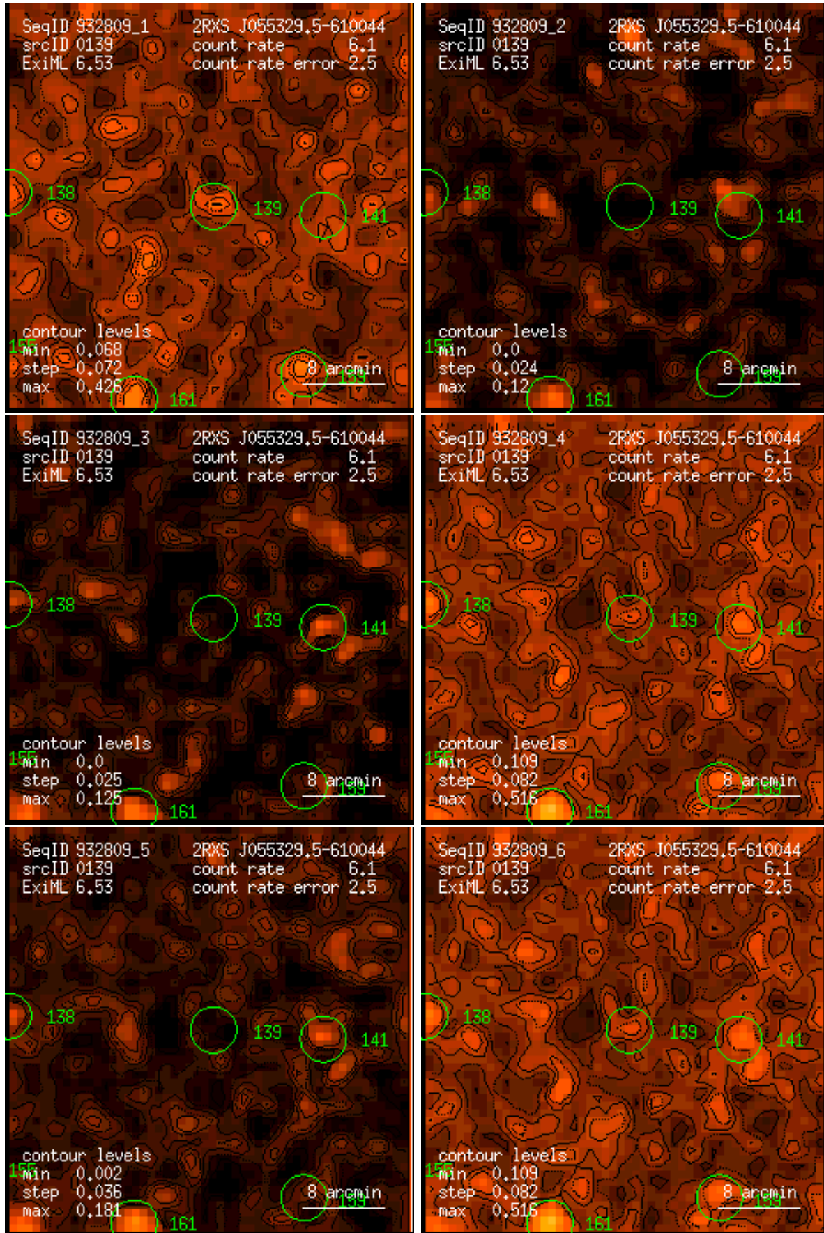
Figure 139: RASS 932809: detection 0139: band rate images, Gaussian filter: (1) PSPC channels 11 – 41, (2) 52 – 90, (3) 91 – 201, (4) 11 – 235, (5) 52 – 201, (6) 11 – 201. Broad band rates in counts/ks. Band rate contour levels in counts/ks/arcmin 2 .
