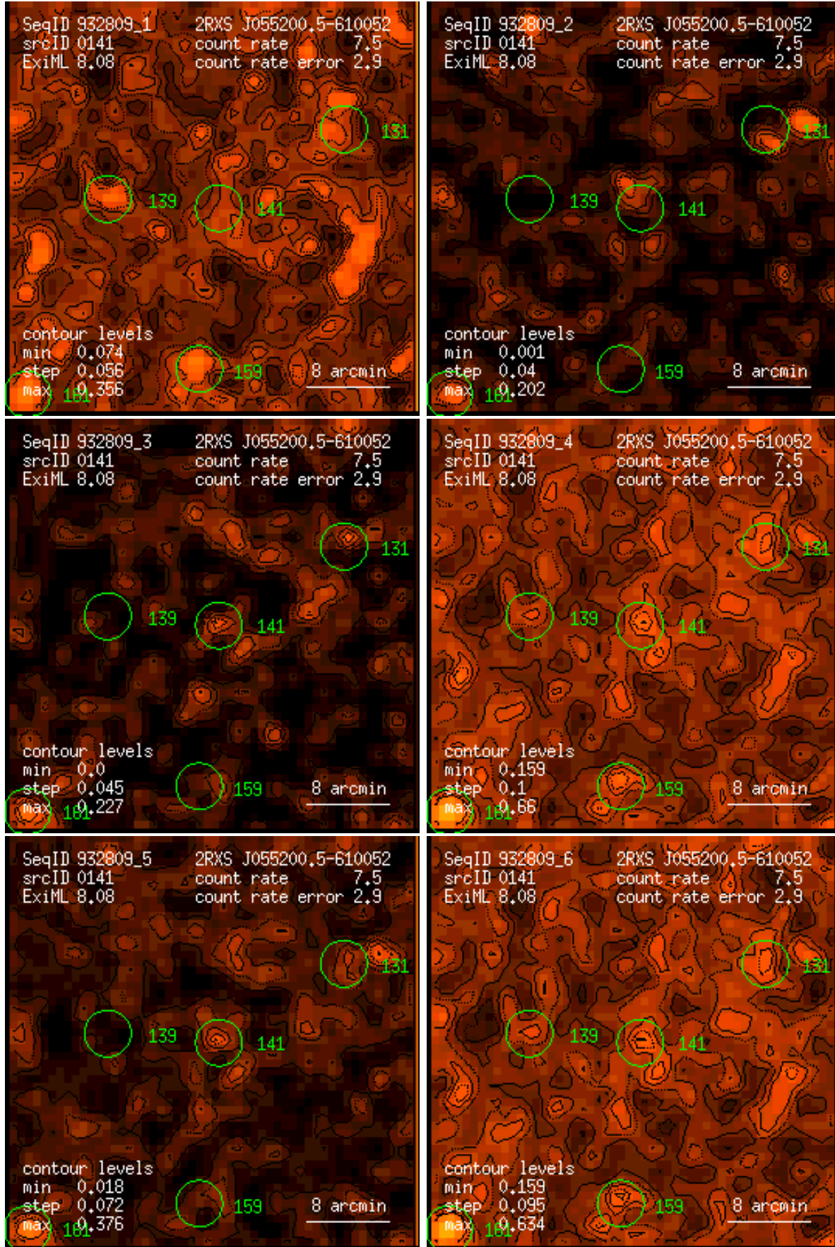
Figure 141: RASS 932809: detection 0141: band rate images, Gaussian filter: (1) PSPC channels 11 – 41, (2) 52 – 90, (3) 91 – 201, (4) 11 – 235, (5) 52 – 201, (6) 11 – 201. Broad band rates in counts/ks. Band rate contour levels in counts/ks/arcmin 2 .
