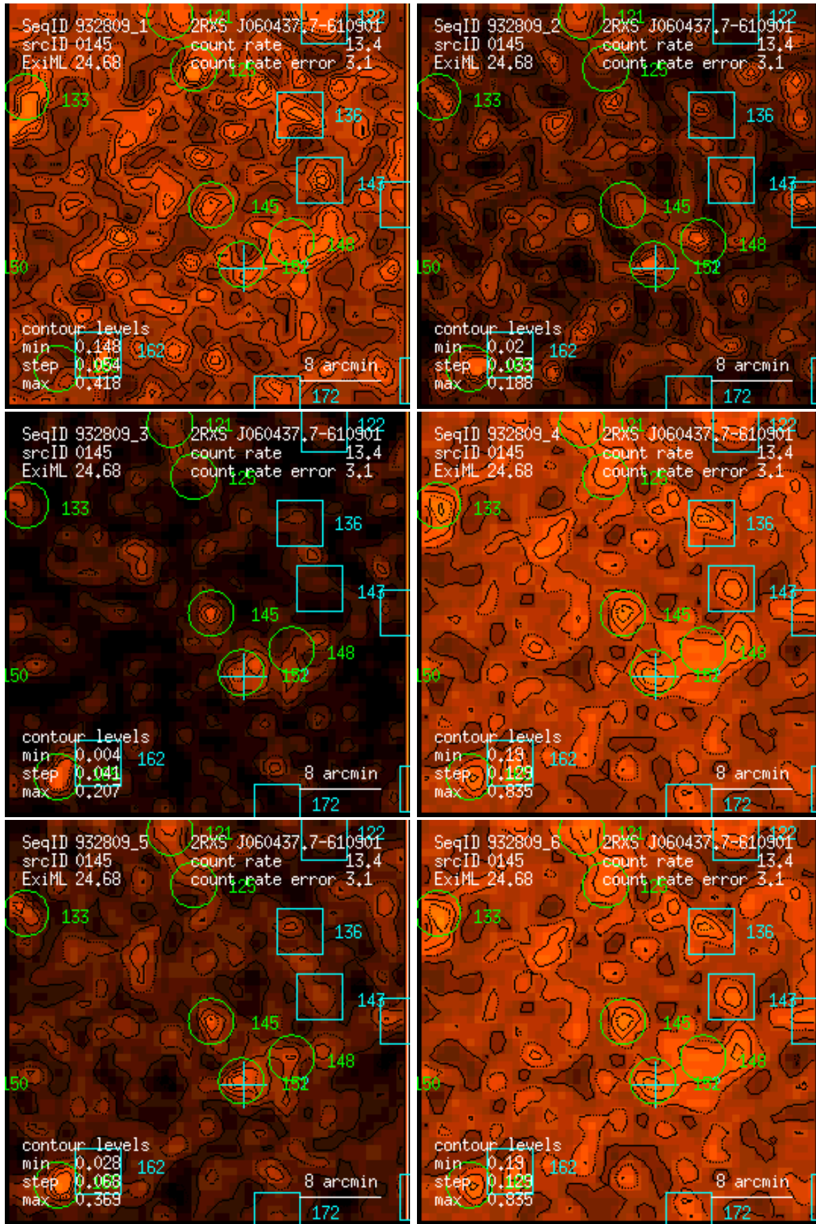
Figure 145: RASS 932809: detection 0145: band rate images, Gaussian filter: (1) PSPC channels 11 – 41, (2) 52 – 90, (3) 91 – 201, (4) 11 – 235, (5) 52 – 201, (6) 11 – 201. Broad band rates in counts/ks. Band rate contour levels in counts/ks/arcmin 2 .
