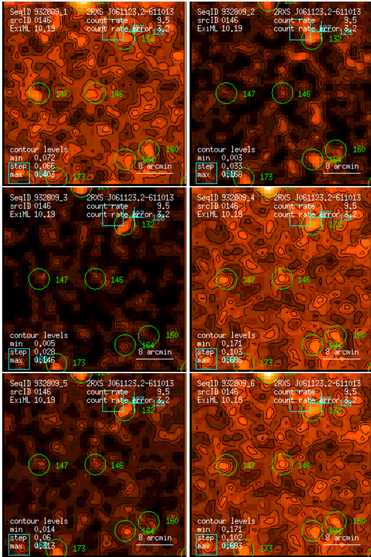
Figure 146: RASS 932809: detection 0146: band rate images, Gaussian filter: (1) PSPC channels 11 – 41, (2) 52 – 90, (3) 91 – 201, (4) 11 – 235, (5) 52 – 201, (6) 11 – 201. Broad band rates in counts/ks. Band rate contour levels in counts/ks/arcmin 2 .
