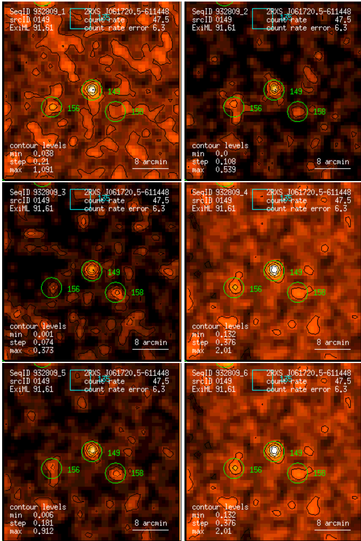
Figure 149: RASS 932809: detection 0149: band rate images, Gaussian filter: (1) PSPC channels 11 – 41, (2) 52 – 90, (3) 91 – 201, (4) 11 – 235, (5) 52 – 201, (6) 11 – 201. Broad band rates in counts/ks. Band rate contour levels in counts/ks/arcmin 2 .
