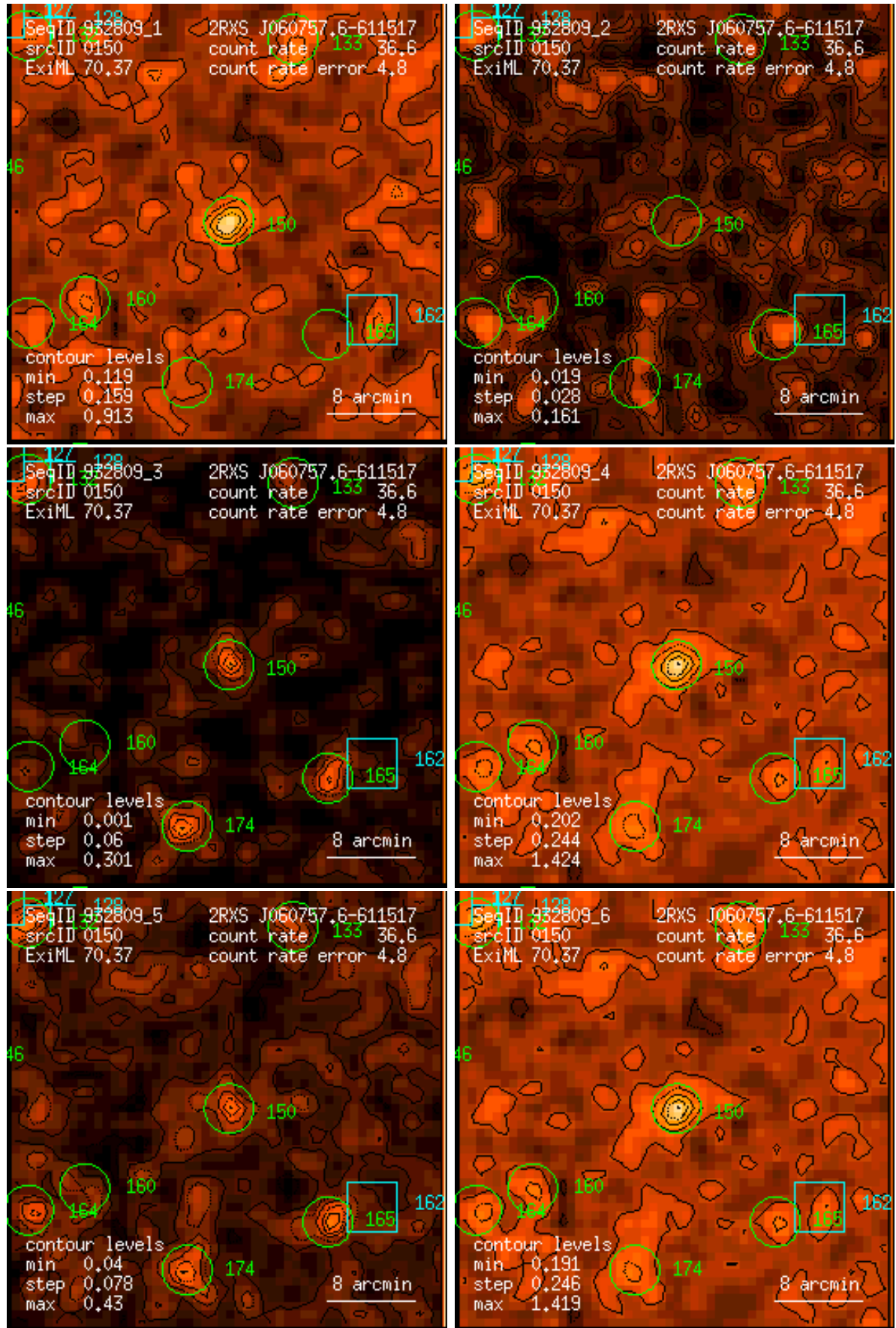
Figure 150: RASS 932809: detection 0150: band rate images, Gaussian filter: (1) PSPC channels 11 – 41, (2) 52 – 90, (3) 91 – 201, (4) 11 – 235, (5) 52 – 201, (6) 11 – 201. Broad band rates in counts/ks. Band rate contour levels in counts/ks/arcmin 2 .
