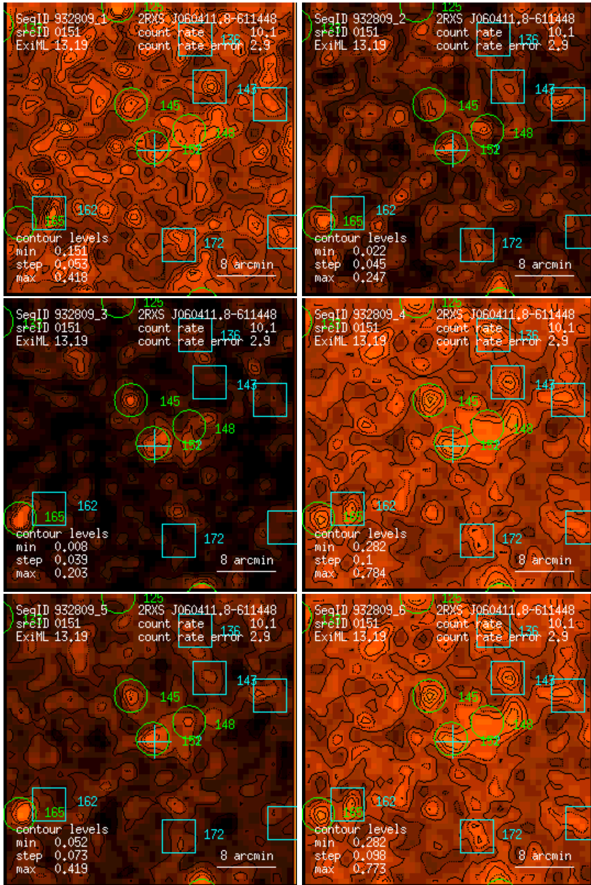
Figure 151: RASS 932809: detection 0151: band rate images, Gaussian filter: (1) PSPC channels 11 – 41, (2) 52 – 90, (3) 91 – 201, (4) 11 – 235, (5) 52 – 201, (6) 11 – 201. Broad band rates in counts/ks. Band rate contour levels in counts/ks/arcmin 2 .
