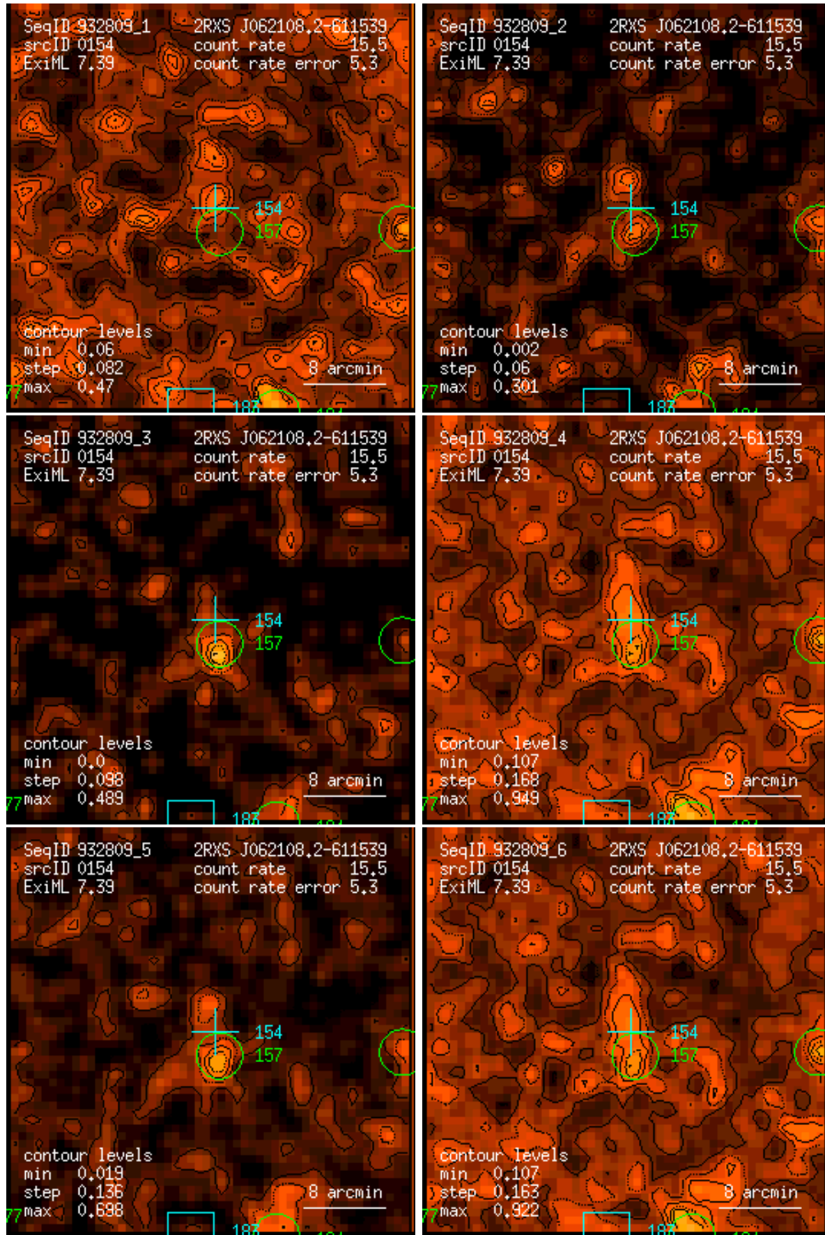
Figure 154: RASS 932809: detection 0154: band rate images, Gaussian filter: (1) PSPC channels 11 – 41, (2) 52 – 90, (3) 91 – 201, (4) 11 – 235, (5) 52 – 201, (6) 11 – 201. Broad band rates in counts/ks. Band rate contour levels in counts/ks/arcmin 2 .
