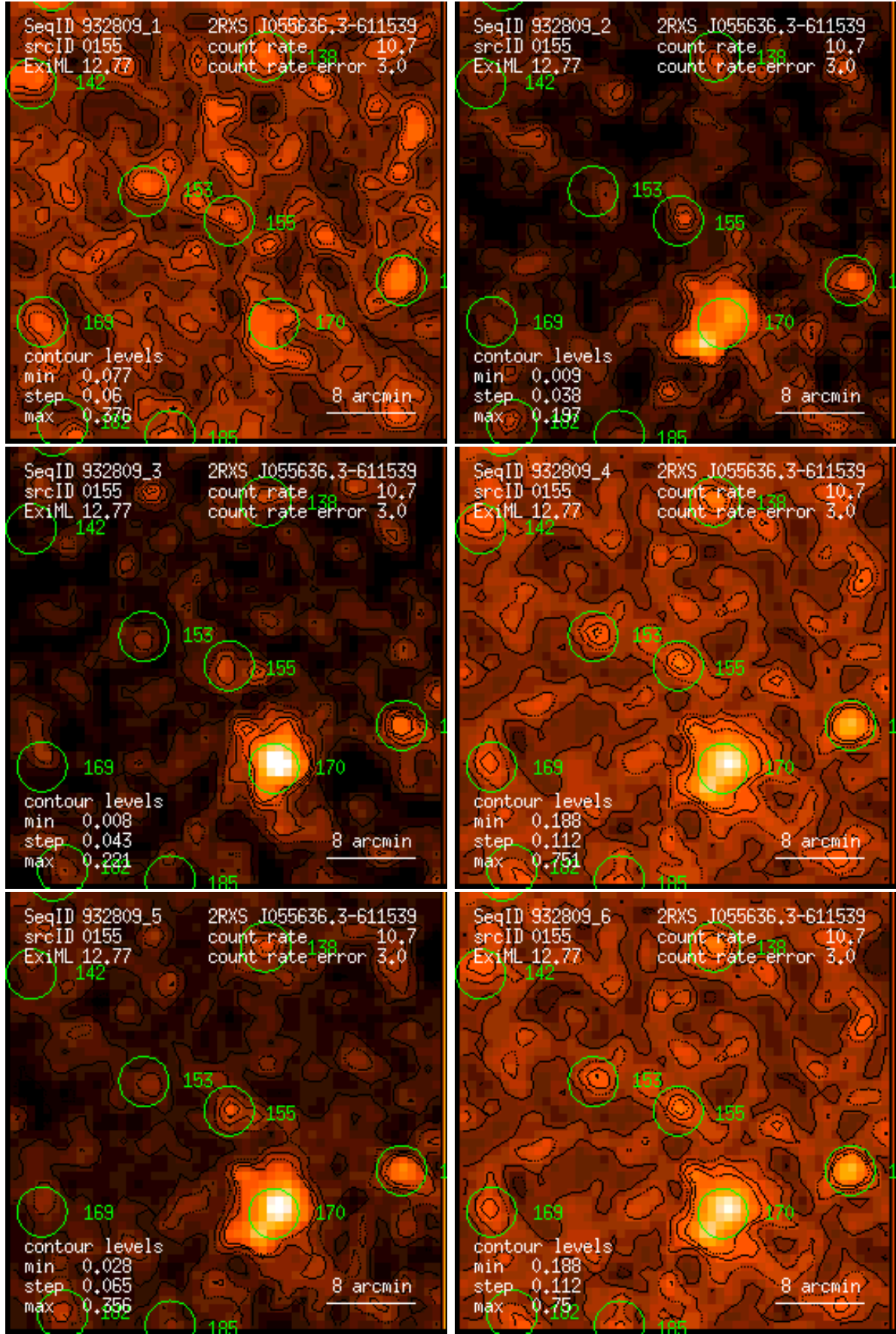
Figure 155: RASS 932809: detection 0155: band rate images, Gaussian filter: (1) PSPC channels 11 – 41, (2) 52 – 90, (3) 91 – 201, (4) 11 – 235, (5) 52 – 201, (6) 11 – 201. Broad band rates in counts/ks. Band rate contour levels in counts/ks/arcmin 2 .
