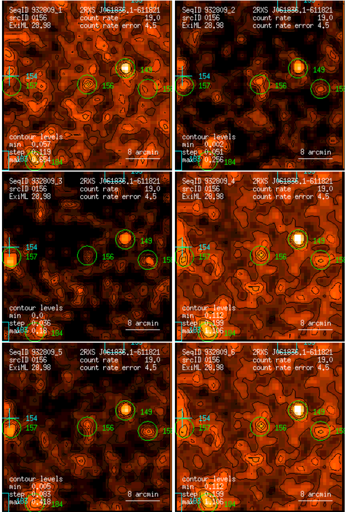
Figure 156: RASS 932809: detection 0156: band rate images, Gaussian filter: (1) PSPC channels 11 – 41, (2) 52 – 90, (3) 91 – 201, (4) 11 – 235, (5) 52 – 201, (6) 11 – 201. Broad band rates in counts/ks. Band rate contour levels in counts/ks/arcmin 2 .
