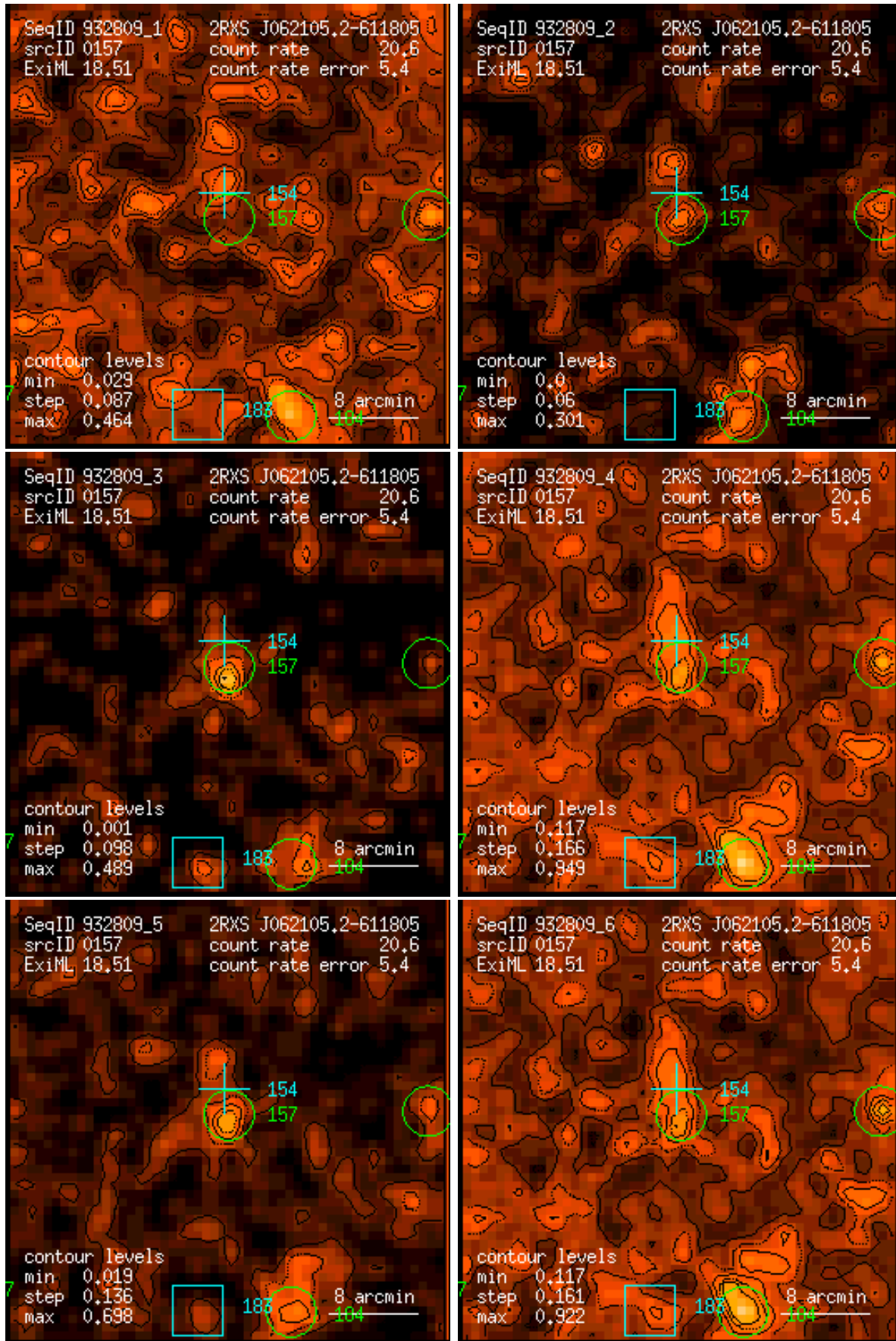
Figure 157: RASS 932809: detection 0157: band rate images, Gaussian filter: (1) PSPC channels 11 – 41, (2) 52 – 90, (3) 91 – 201, (4) 11 – 235, (5) 52 – 201, (6) 11 – 201. Broad band rates in counts/ks. Band rate contour levels in counts/ks/arcmin 2 .
