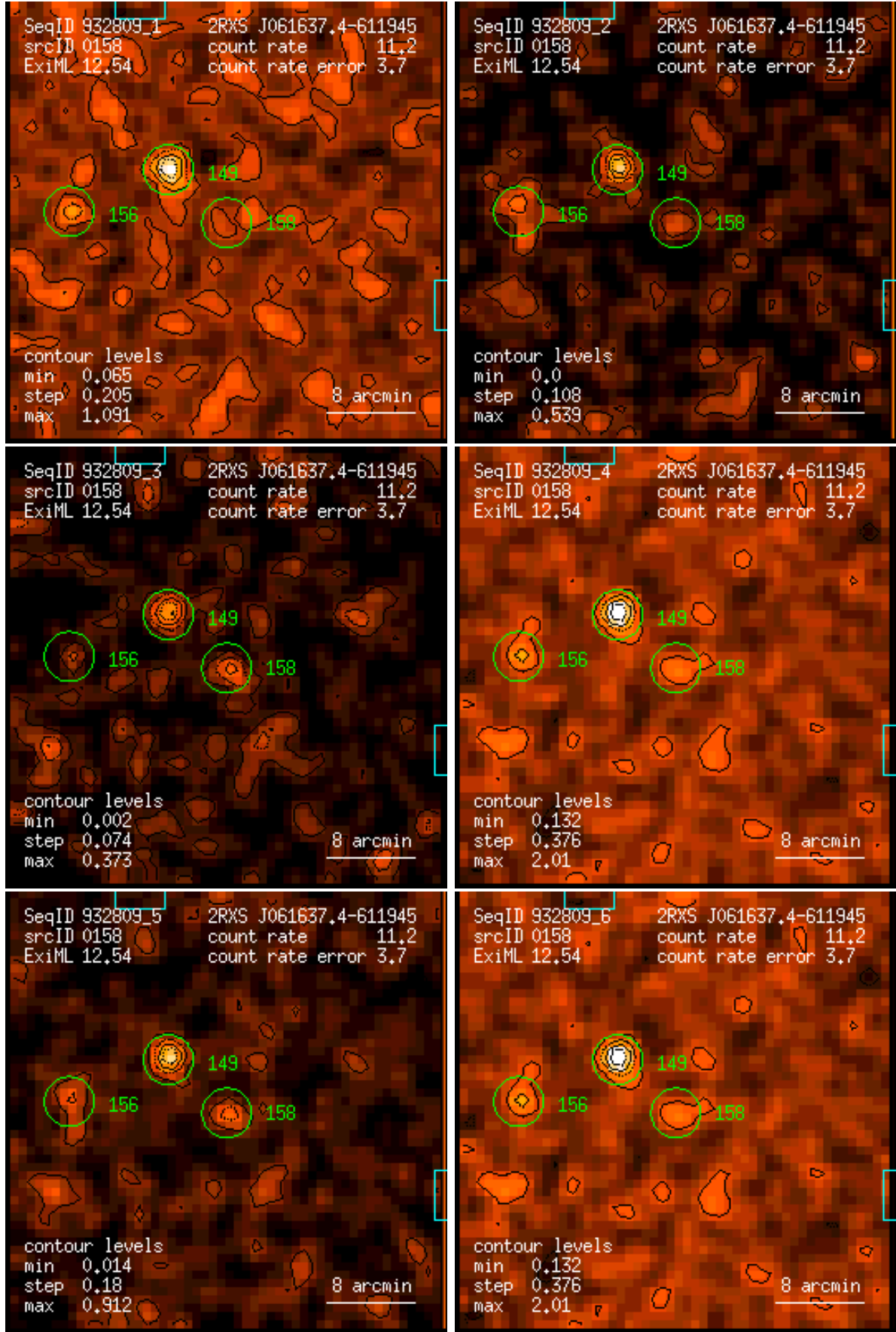
Figure 158: RASS 932809: detection 0158: band rate images, Gaussian filter: (1) PSPC channels 11 – 41, (2) 52 – 90, (3) 91 – 201, (4) 11 – 235, (5) 52 – 201, (6) 11 – 201. Broad band rates in counts/ks. Band rate contour levels in counts/ks/arcmin 2 .
