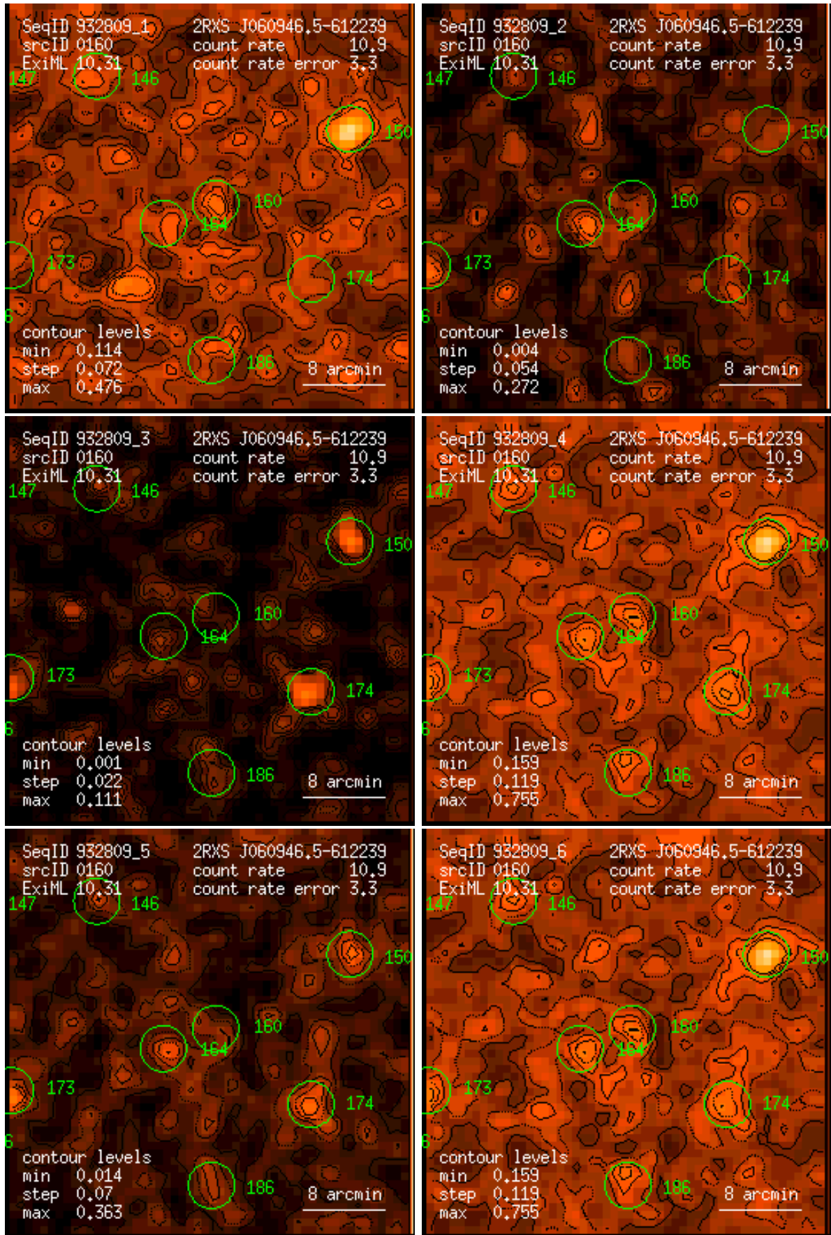
Figure 160: RASS 932809: detection 0160: band rate images, Gaussian filter: (1) PSPC channels 11 – 41, (2) 52 – 90, (3) 91 – 201, (4) 11 – 235, (5) 52 – 201, (6) 11 – 201. Broad band rates in counts/ks. Band rate contour levels in counts/ks/arcmin 2 .
