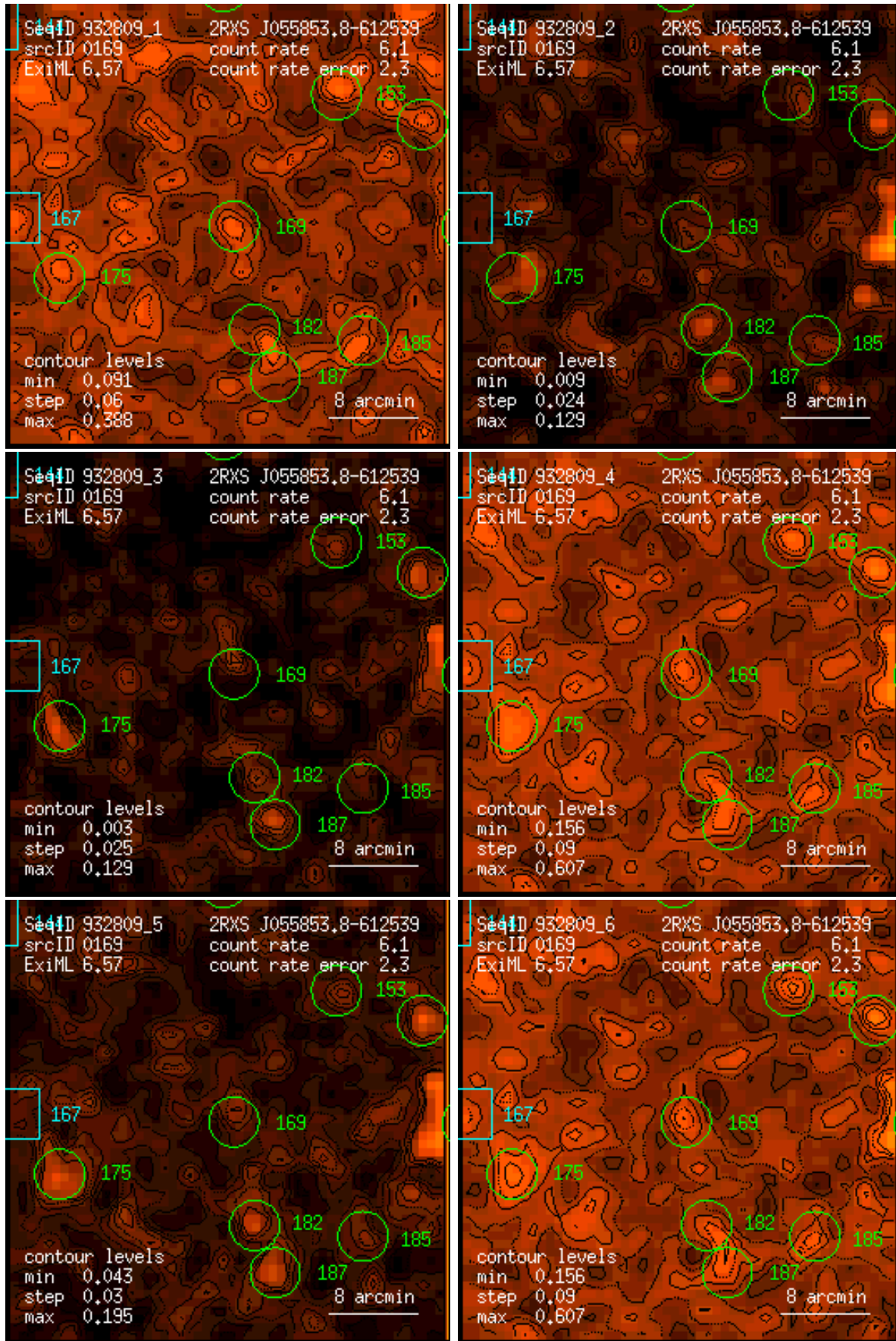
Figure 169: RASS 932809: detection 0169: band rate images, Gaussian filter: (1) PSPC channels 11 – 41, (2) 52 – 90, (3) 91 – 201, (4) 11 – 235, (5) 52 – 201, (6) 11 – 201. Broad band rates in counts/ks. Band rate contour levels in counts/ks/arcmin 2 .
