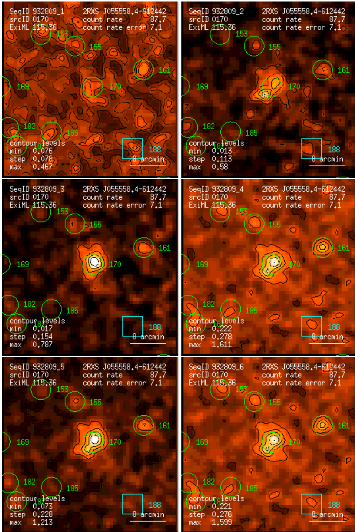
Figure 170: RASS 932809: detection 0170: band rate images, Gaussian filter: (1) PSPC channels 11 – 41, (2) 52 – 90, (3) 91 – 201, (4) 11 – 235, (5) 52 – 201, (6) 11 – 201. Broad band rates in counts/ks. Band rate contour levels in counts/ks/arcmin 2 .
