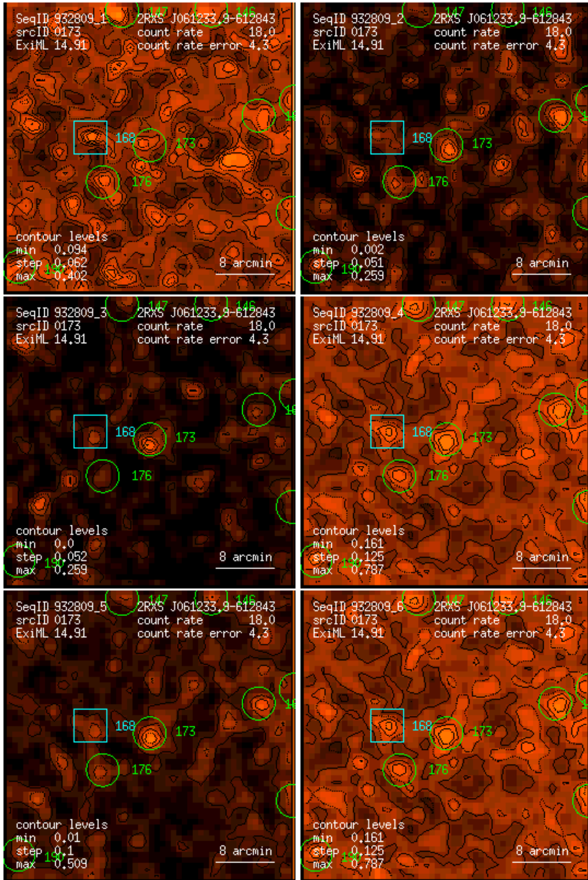
Figure 173: RASS 932809: detection 0173: band rate images, Gaussian filter: (1) PSPC channels 11 – 41, (2) 52 – 90, (3) 91 – 201, (4) 11 – 235, (5) 52 – 201, (6) 11 – 201. Broad band rates in counts/ks. Band rate contour levels in counts/ks/arcmin 2 .
