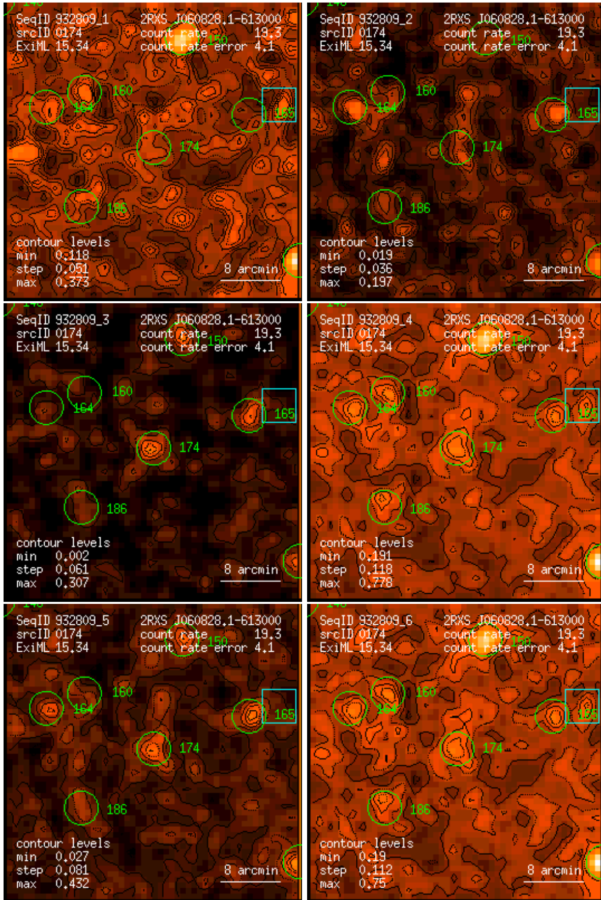
Figure 174: RASS 932809: detection 0174: band rate images, Gaussian filter: (1) PSPC channels 11 – 41, (2) 52 – 90, (3) 91 – 201, (4) 11 – 235, (5) 52 – 201, (6) 11 – 201. Broad band rates in counts/ks. Band rate contour levels in counts/ks/arcmin 2 .
