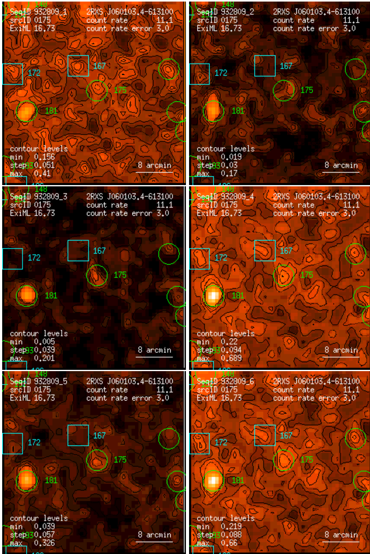
Figure 175: RASS 932809: detection 0175: band rate images, Gaussian filter: (1) PSPC channels 11 – 41, (2) 52 – 90, (3) 91 – 201, (4) 11 – 235, (5) 52 – 201, (6) 11 – 201. Broad band rates in counts/ks. Band rate contour levels in counts/ks/arcmin 2 .
