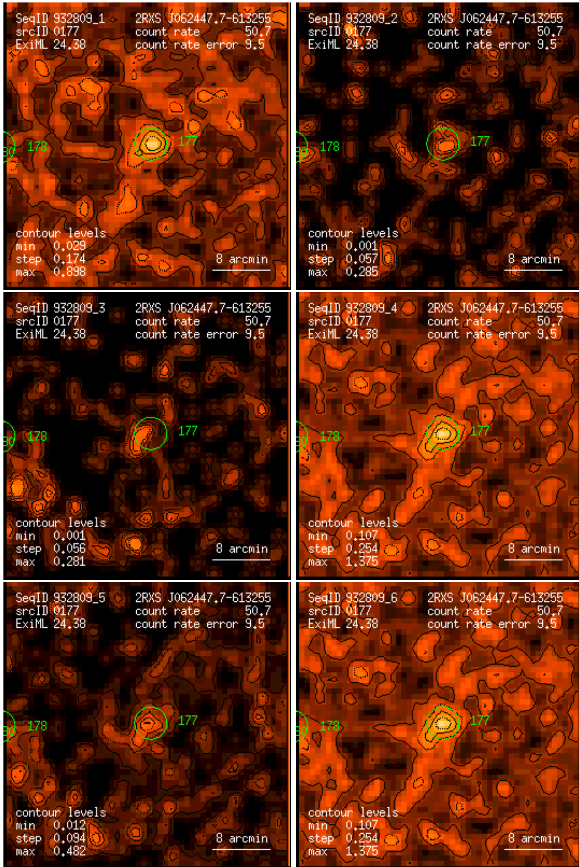
Figure 177: RASS 932809: detection 0177: band rate images, Gaussian filter: (1) PSPC channels 11 – 41, (2) 52 – 90, (3) 91 – 201, (4) 11 – 235, (5) 52 – 201, (6) 11 – 201. Broad band rates in counts/ks. Band rate contour levels in counts/ks/arcmin 2 .
