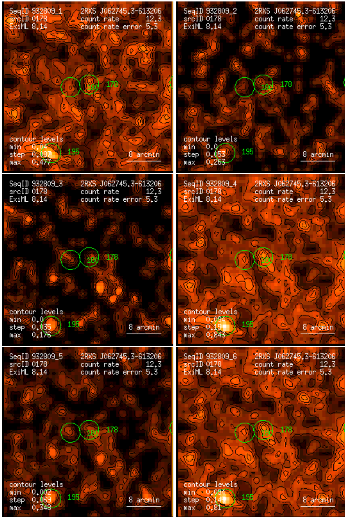
Figure 178: RASS 932809: detection 0178: band rate images, Gaussian filter: (1) PSPC channels 11 – 41, (2) 52 – 90, (3) 91 – 201, (4) 11 – 235, (5) 52 – 201, (6) 11 – 201. Broad band rates in counts/ks. Band rate contour levels in counts/ks/arcmin 2 .
