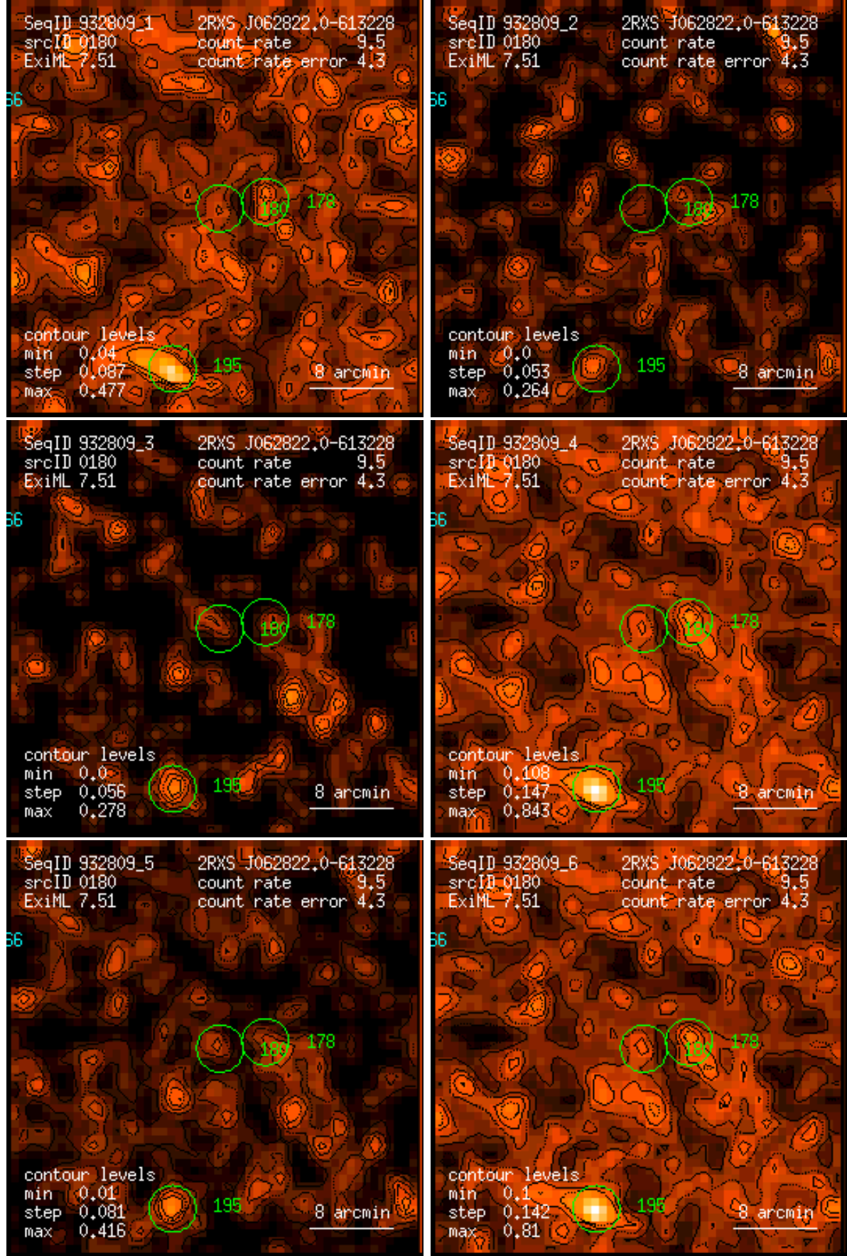
Figure 180: RASS 932809: detection 0180: band rate images, Gaussian filter: (1) PSPC channels 11 – 41, (2) 52 – 90, (3) 91 – 201, (4) 11 – 235, (5) 52 – 201, (6) 11 – 201. Broad band rates in counts/ks. Band rate contour levels in counts/ks/arcmin 2 .
