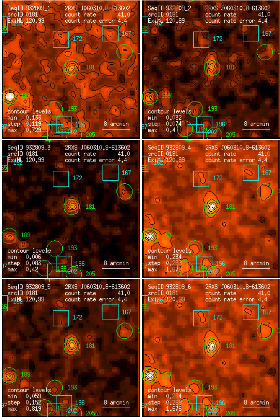
Figure 181: RASS 932809: detection 0181: band rate images, Gaussian filter: (1) PSPC channels 11 – 41, (2) 52 – 90, (3) 91 – 201, (4) 11 – 235, (5) 52 – 201, (6) 11 – 201. Broad band rates in counts/ks. Band rate contour levels in counts/ks/arcmin 2 .
