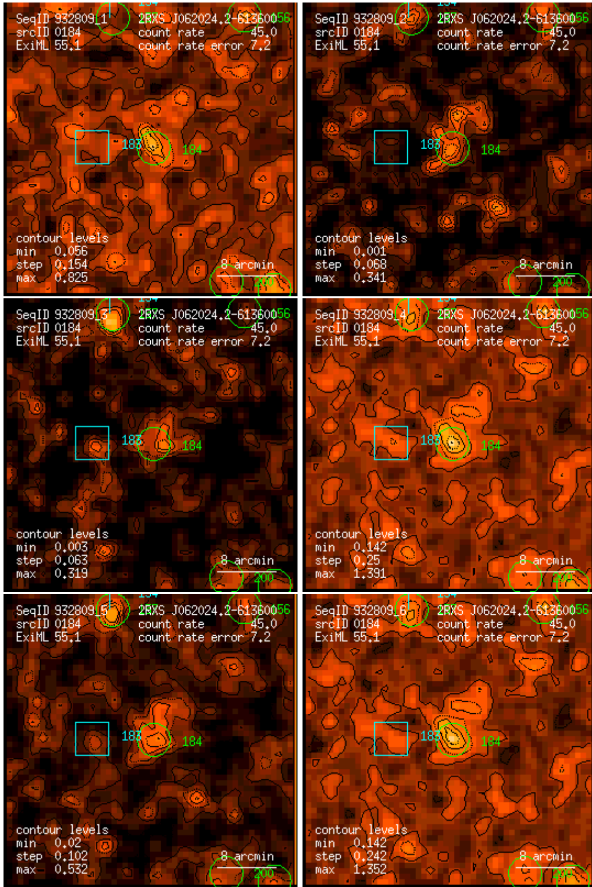
Figure 184: RASS 932809: detection 0184: band rate images, Gaussian filter: (1) PSPC channels 11 – 41, (2) 52 – 90, (3) 91 – 201, (4) 11 – 235, (5) 52 – 201, (6) 11 – 201. Broad band rates in counts/ks. Band rate contour levels in counts/ks/arcmin 2 .
