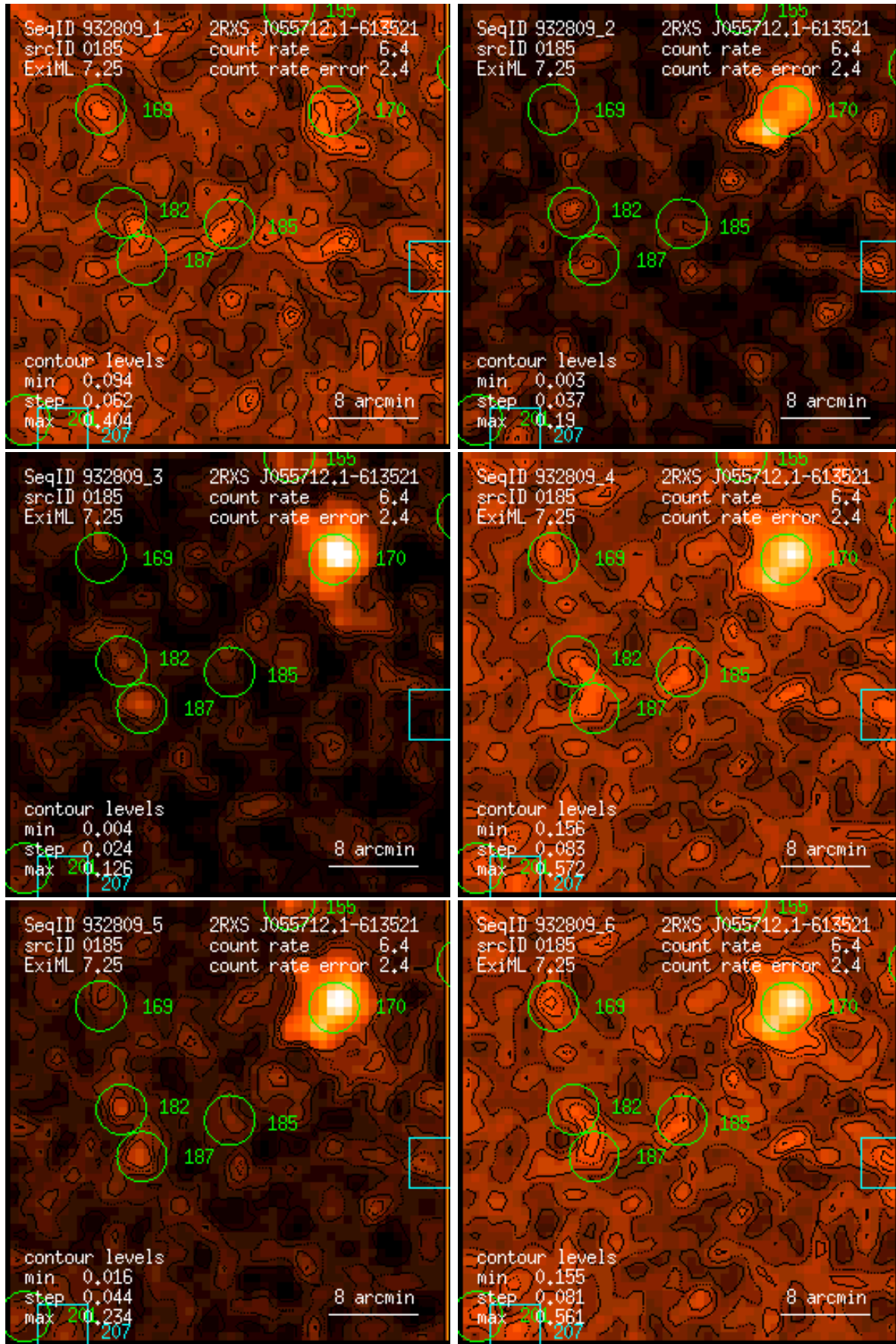
Figure 185: RASS 932809: detection 0185: band rate images, Gaussian filter: (1) PSPC channels 11 – 41, (2) 52 – 90, (3) 91 – 201, (4) 11 – 235, (5) 52 – 201, (6) 11 – 201. Broad band rates in counts/ks. Band rate contour levels in counts/ks/arcmin 2 .
