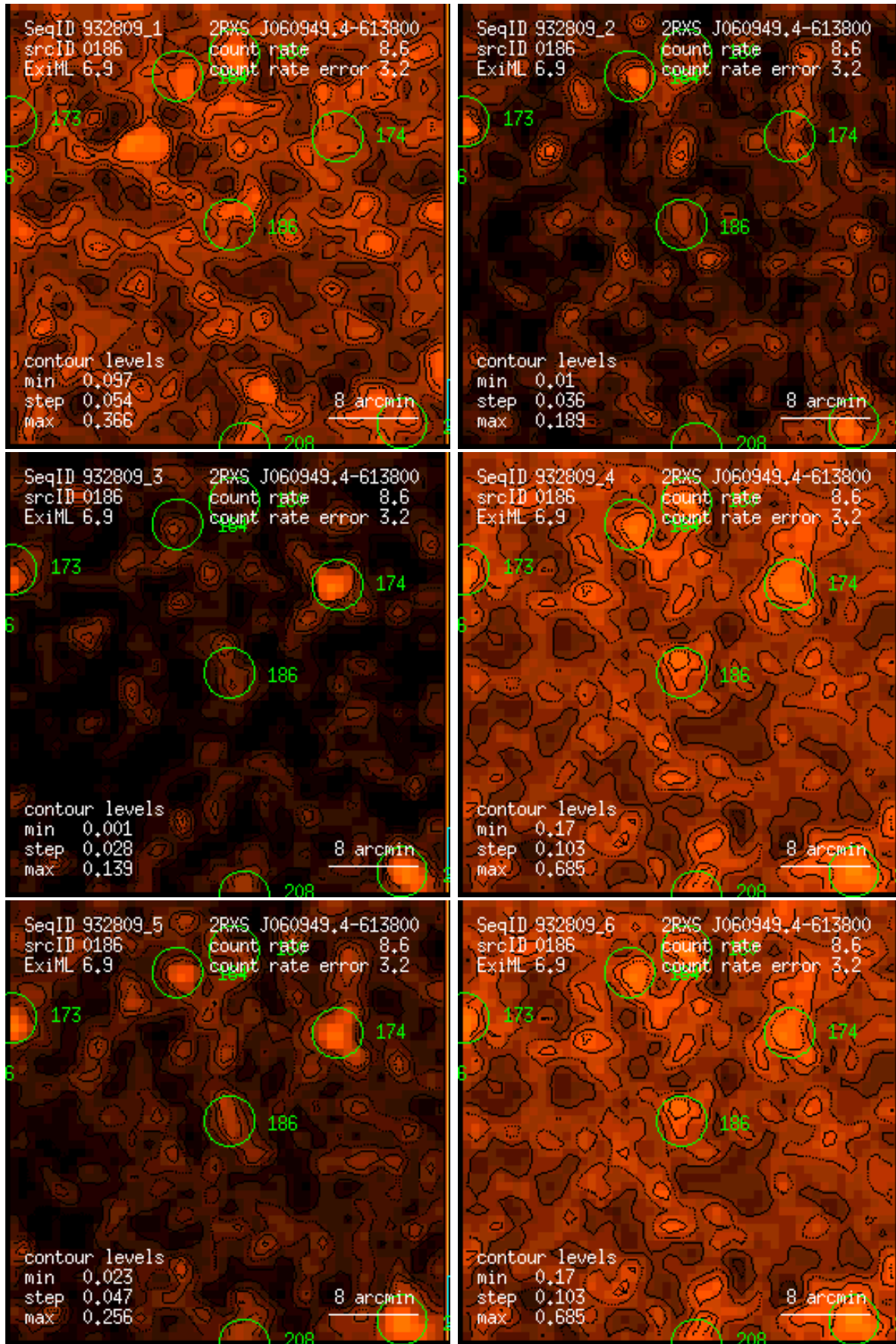
Figure 186: RASS 932809: detection 0186: band rate images, Gaussian filter: (1) PSPC channels 11 – 41, (2) 52 – 90, (3) 91 – 201, (4) 11 – 235, (5) 52 – 201, (6) 11 – 201. Broad band rates in counts/ks. Band rate contour levels in counts/ks/arcmin 2 .
