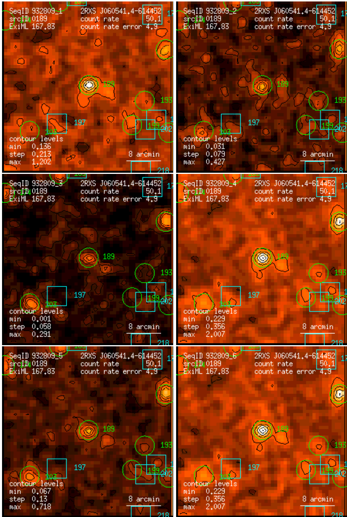
Figure 189: RASS 932809: detection 0189: band rate images, Gaussian filter: (1) PSPC channels 11 – 41, (2) 52 – 90, (3) 91 – 201, (4) 11 – 235, (5) 52 – 201, (6) 11 – 201. Broad band rates in counts/ks. Band rate contour levels in counts/ks/arcmin 2 .
