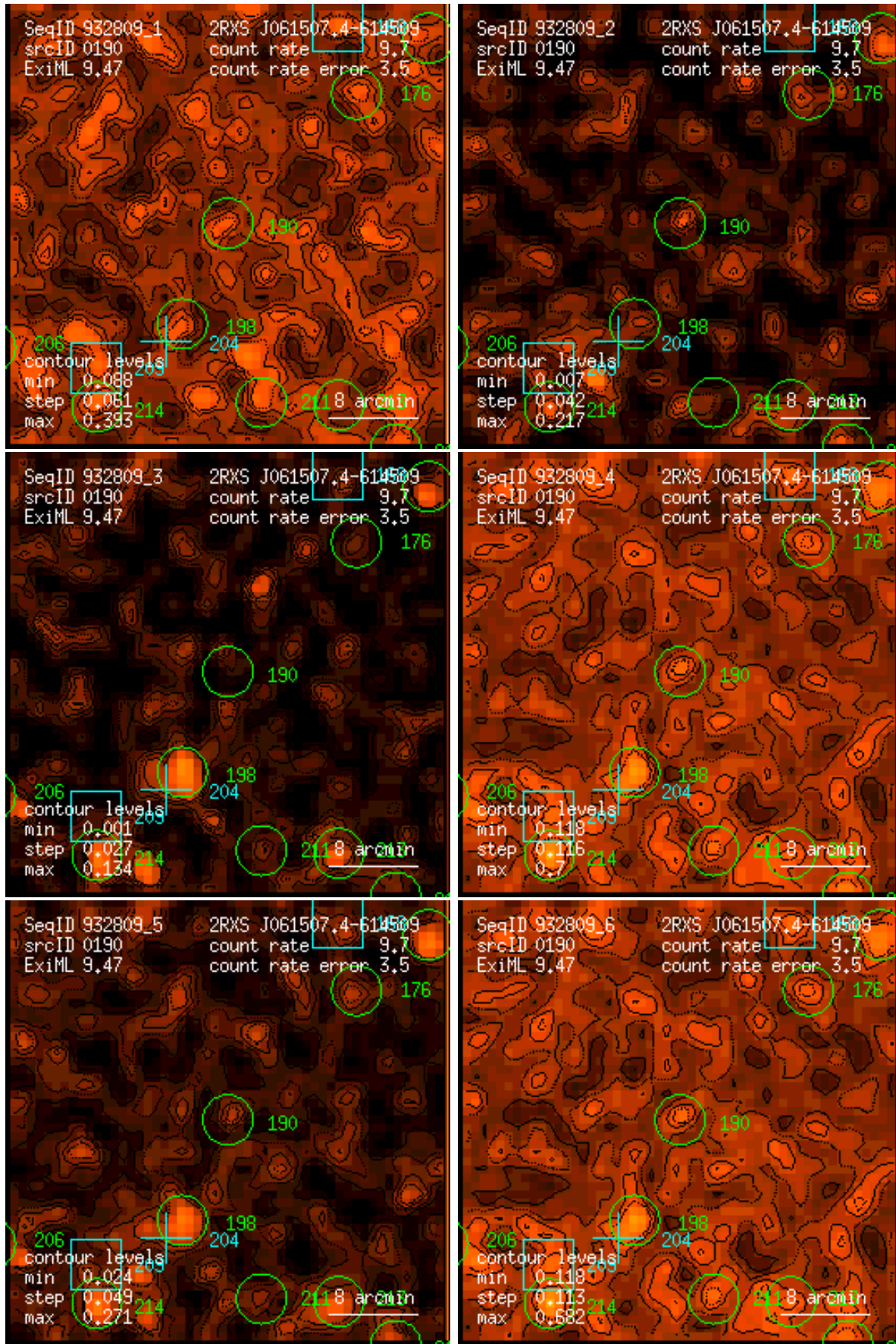
Figure 190: RASS 932809: detection 0190: band rate images, Gaussian filter: (1) PSPC channels 11 – 41, (2) 52 – 90, (3) 91 – 201, (4) 11 – 235, (5) 52 – 201, (6) 11 – 201. Broad band rates in counts/ks. Band rate contour levels in counts/ks/arcmin 2 .
