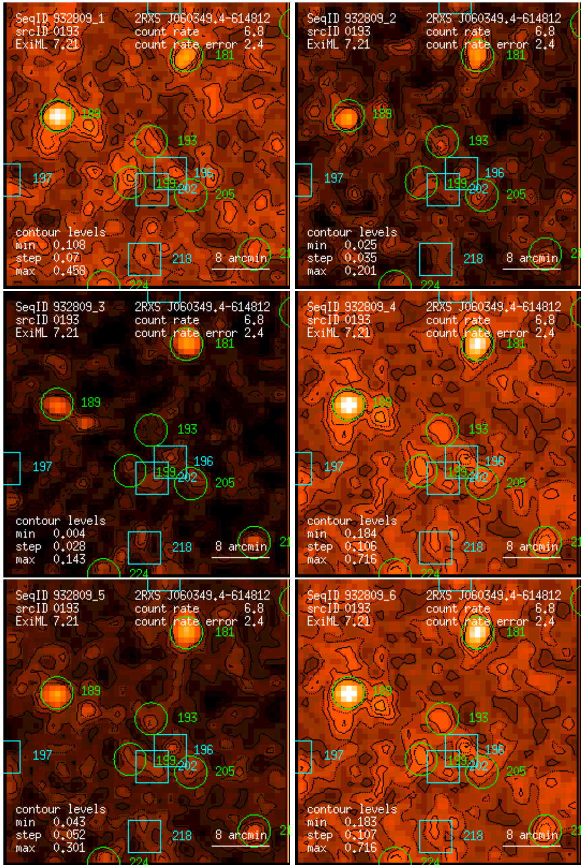
Figure 193: RASS 932809: detection 0193: band rate images, Gaussian filter: (1) PSPC channels 11 – 41, (2) 52 – 90, (3) 91 – 201, (4) 11 – 235, (5) 52 – 201, (6) 11 – 201. Broad band rates in counts/ks. Band rate contour levels in counts/ks/arcmin 2 .
