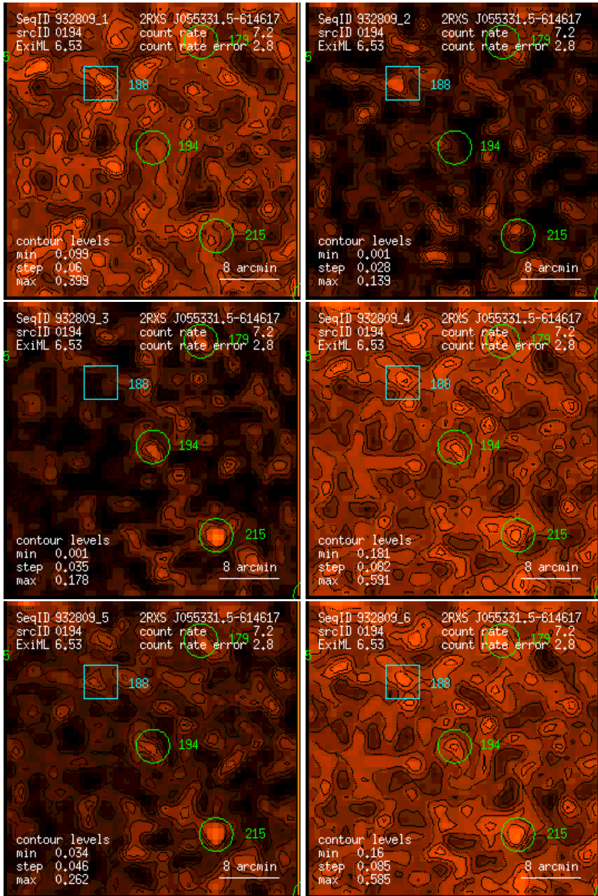
Figure 194: RASS 932809: detection 0194: band rate images, Gaussian filter: (1) PSPC channels 11 – 41, (2) 52 – 90, (3) 91 – 201, (4) 11 – 235, (5) 52 – 201, (6) 11 – 201. Broad band rates in counts/ks. Band rate contour levels in counts/ks/arcmin 2 .
