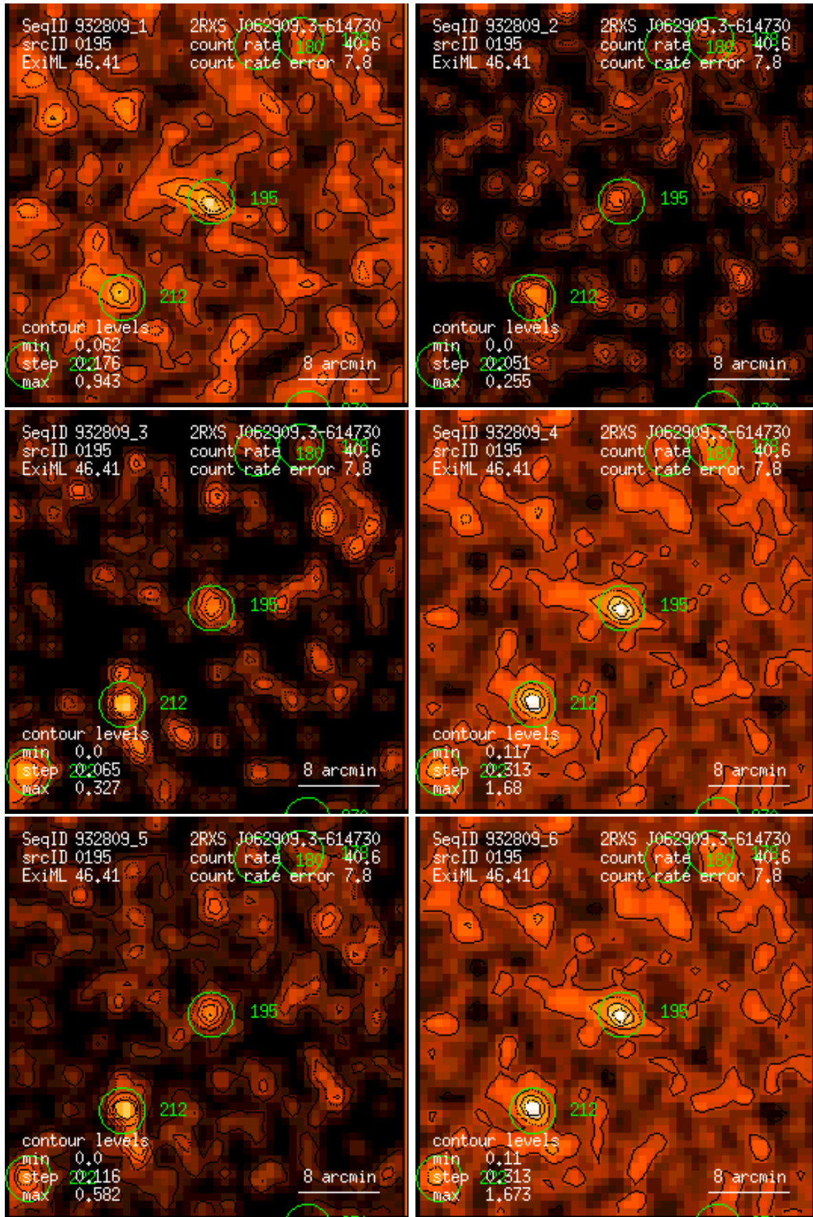
Figure 195: RASS 932809: detection 0195: band rate images, Gaussian filter: (1) PSPC channels 11 – 41, (2) 52 – 90, (3) 91 – 201, (4) 11 – 235, (5) 52 – 201, (6) 11 – 201. Broad band rates in counts/ks. Band rate contour levels in counts/ks/arcmin 2 .
