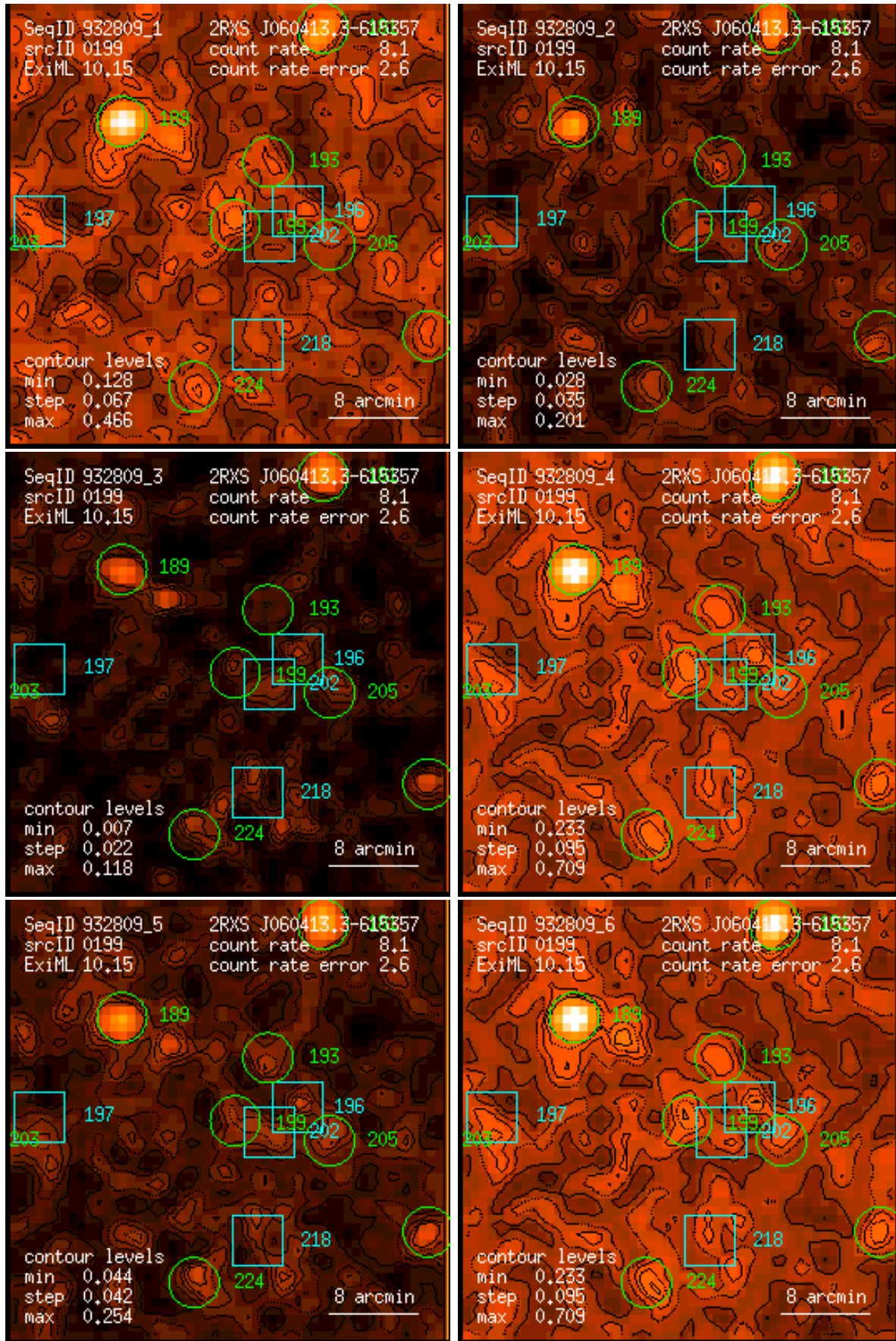
Figure 199: RASS 932809: detection 0199: band rate images, Gaussian filter: (1) PSPC channels 11 – 41, (2) 52 – 90, (3) 91 – 201, (4) 11 – 235, (5) 52 – 201, (6) 11 – 201. Broad band rates in counts/ks. Band rate contour levels in counts/ks/arcmin 2 .
