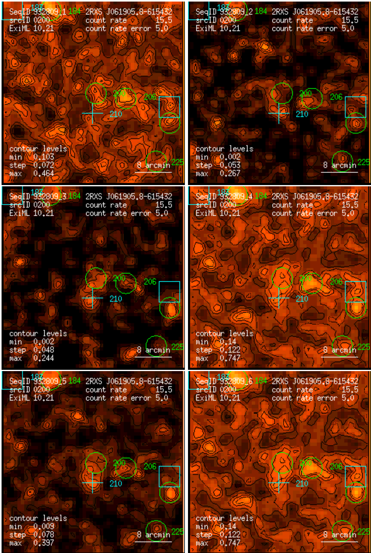
Figure 200: RASS 932809: detection 0200: band rate images, Gaussian filter: (1) PSPC channels 11 – 41, (2) 52 – 90, (3) 91 – 201, (4) 11 – 235, (5) 52 – 201, (6) 11 – 201. Broad band rates in counts/ks. Band rate contour levels in counts/ks/arcmin 2 .
