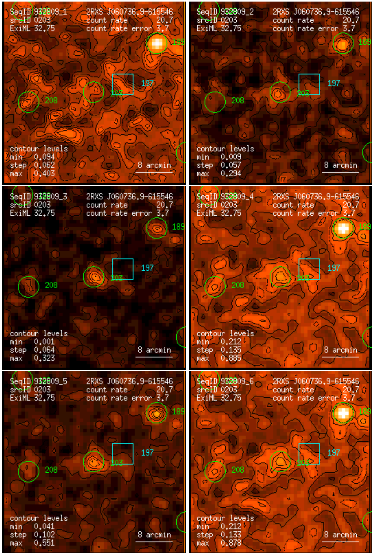
Figure 203: RASS 932809: detection 0203: band rate images, Gaussian filter: (1) PSPC channels 11 – 41, (2) 52 – 90, (3) 91 – 201, (4) 11 – 235, (5) 52 – 201, (6) 11 – 201. Broad band rates in counts/ks. Band rate contour levels in counts/ks/arcmin 2 .
