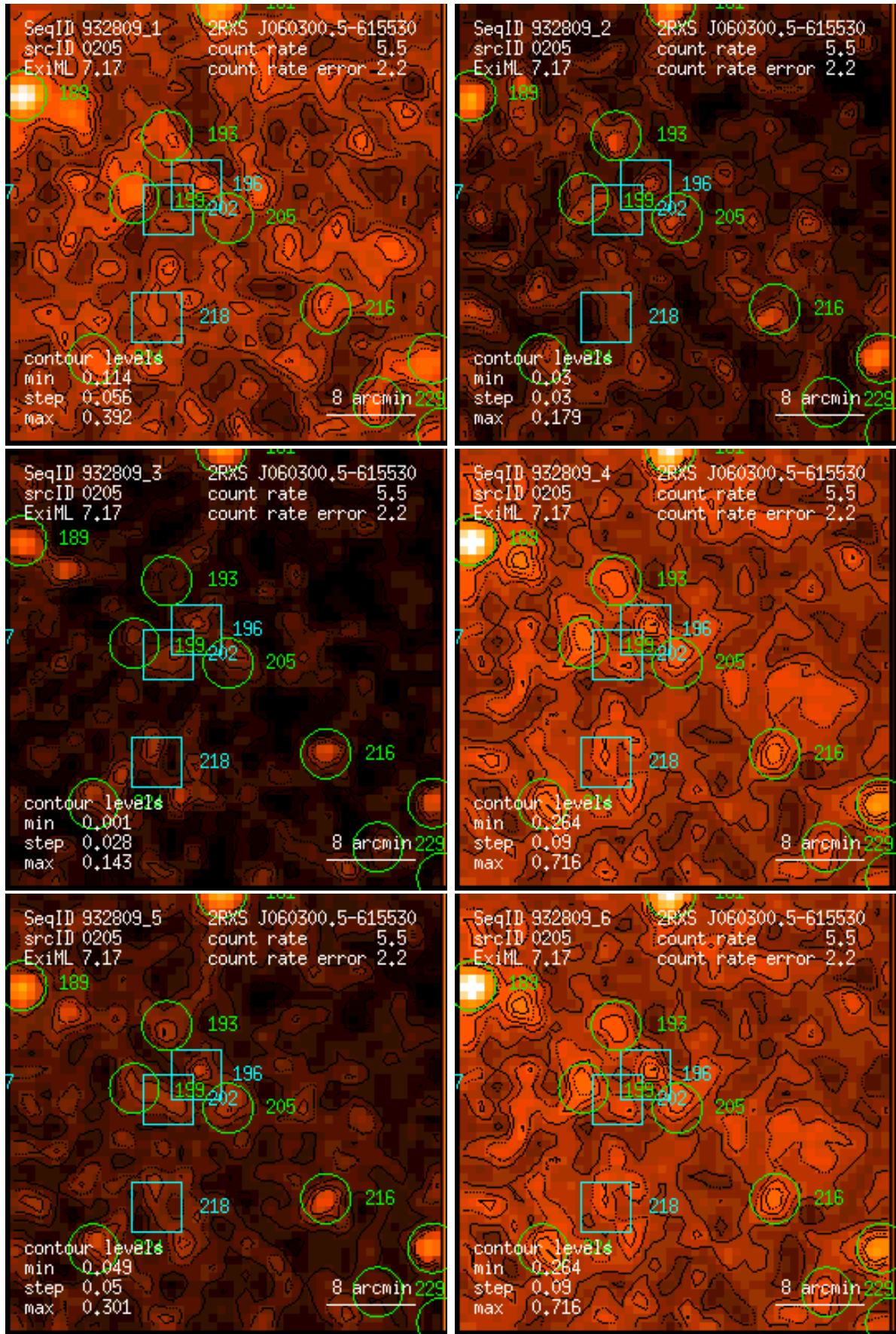
Figure 205: RASS 932809: detection 0205: band rate images, Gaussian filter: (1) PSPC channels 11 – 41, (2) 52 – 90, (3) 91 – 201, (4) 11 – 235, (5) 52 – 201, (6) 11 – 201. Broad band rates in counts/ks. Band rate contour levels in counts/ks/arcmin 2 .
