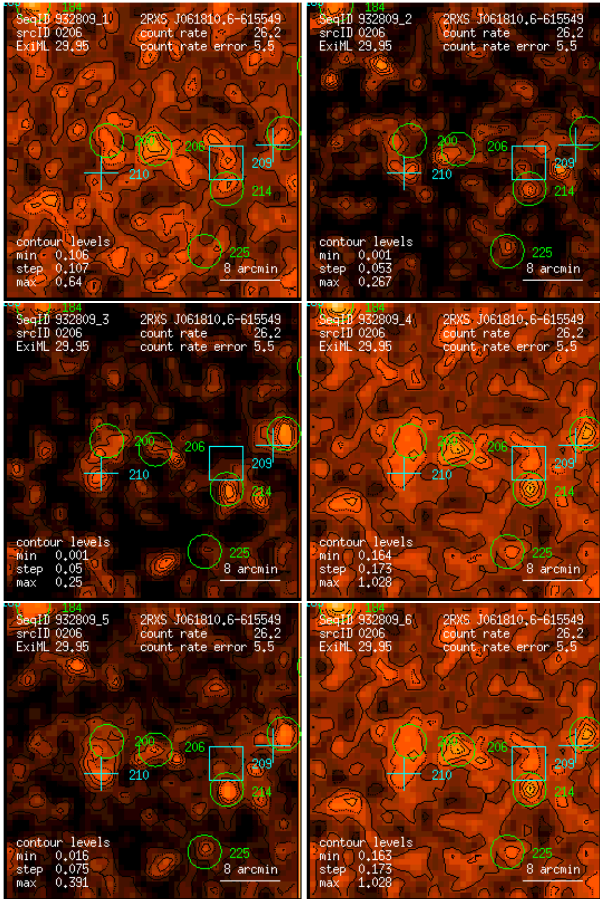
Figure 206: RASS 932809: detection 0206: band rate images, Gaussian filter: (1) PSPC channels 11 – 41, (2) 52 – 90, (3) 91 – 201, (4) 11 – 235, (5) 52 – 201, (6) 11 – 201. Broad band rates in counts/ks. Band rate contour levels in counts/ks/arcmin 2 .
