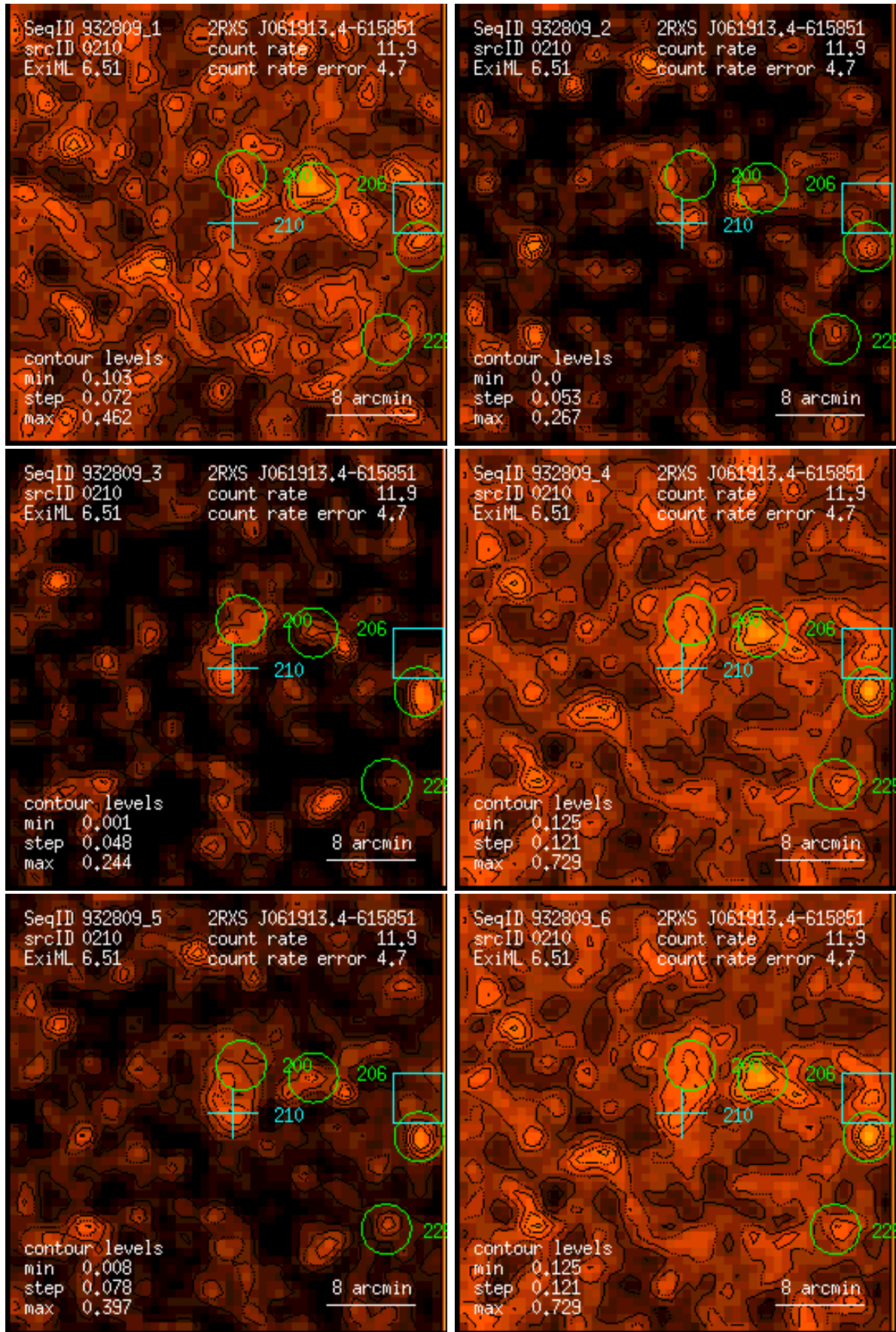
Figure 210: RASS 932809: detection 0210: band rate images, Gaussian filter: (1) PSPC channels 11 – 41, (2) 52 – 90, (3) 91 – 201, (4) 11 – 235, (5) 52 – 201, (6) 11 – 201. Broad band rates in counts/ks. Band rate contour levels in counts/ks/arcmin 2 .
