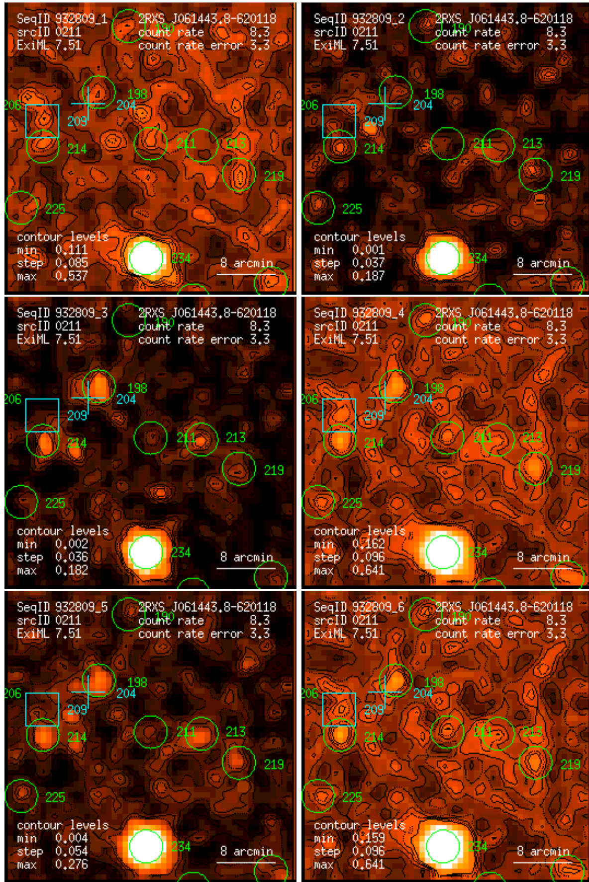
Figure 211: RASS 932809: detection 0211: band rate images, Gaussian filter: (1) PSPC channels 11 – 41, (2) 52 – 90, (3) 91 – 201, (4) 11 – 235, (5) 52 – 201, (6) 11 – 201. Broad band rates in counts/ks. Band rate contour levels in counts/ks/arcmin 2 .
