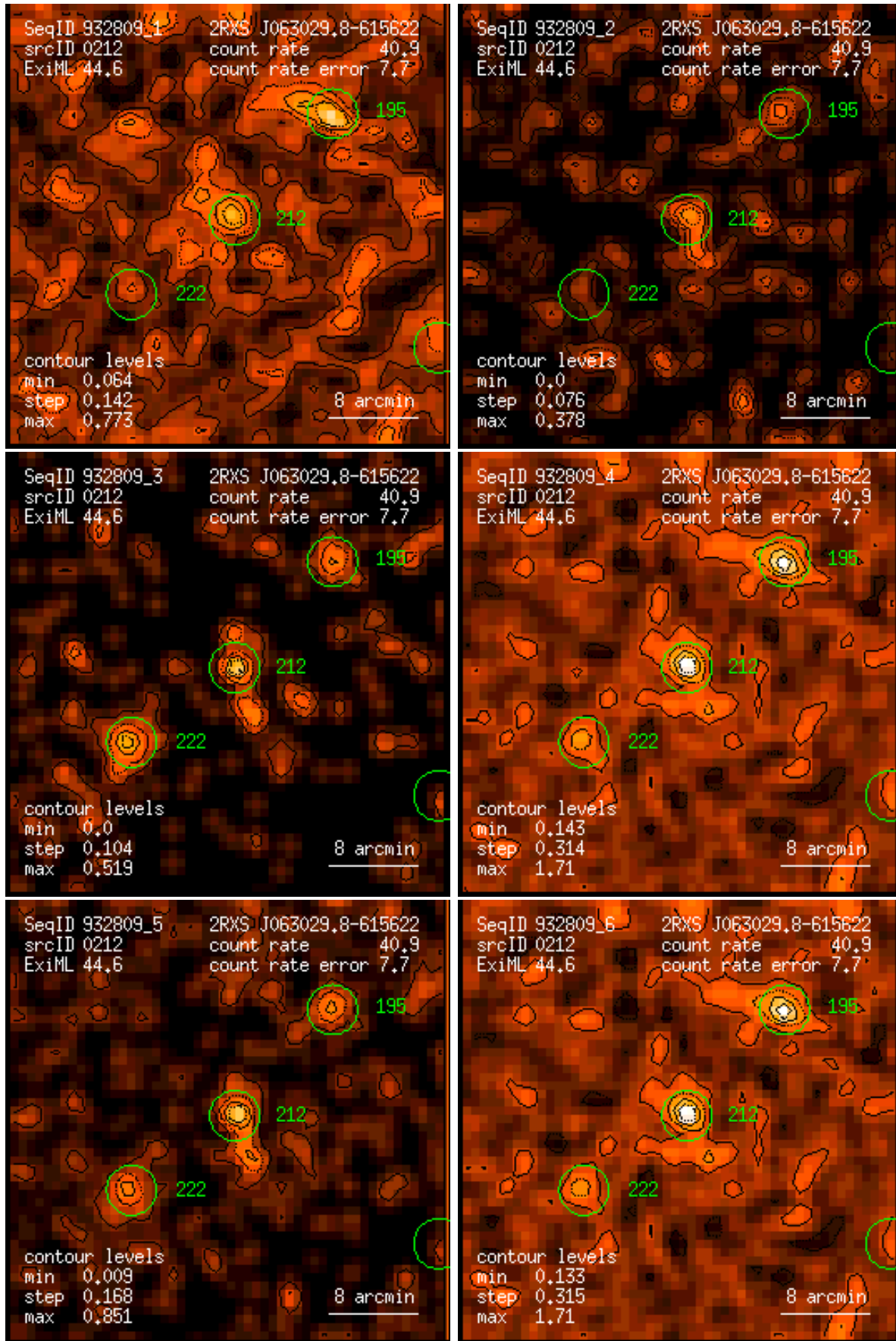
Figure 212: RASS 932809: detection 0212: band rate images, Gaussian filter: (1) PSPC channels 11 – 41, (2) 52 – 90, (3) 91 – 201, (4) 11 – 235, (5) 52 – 201, (6) 11 – 201. Broad band rates in counts/ks. Band rate contour levels in counts/ks/arcmin 2 .
