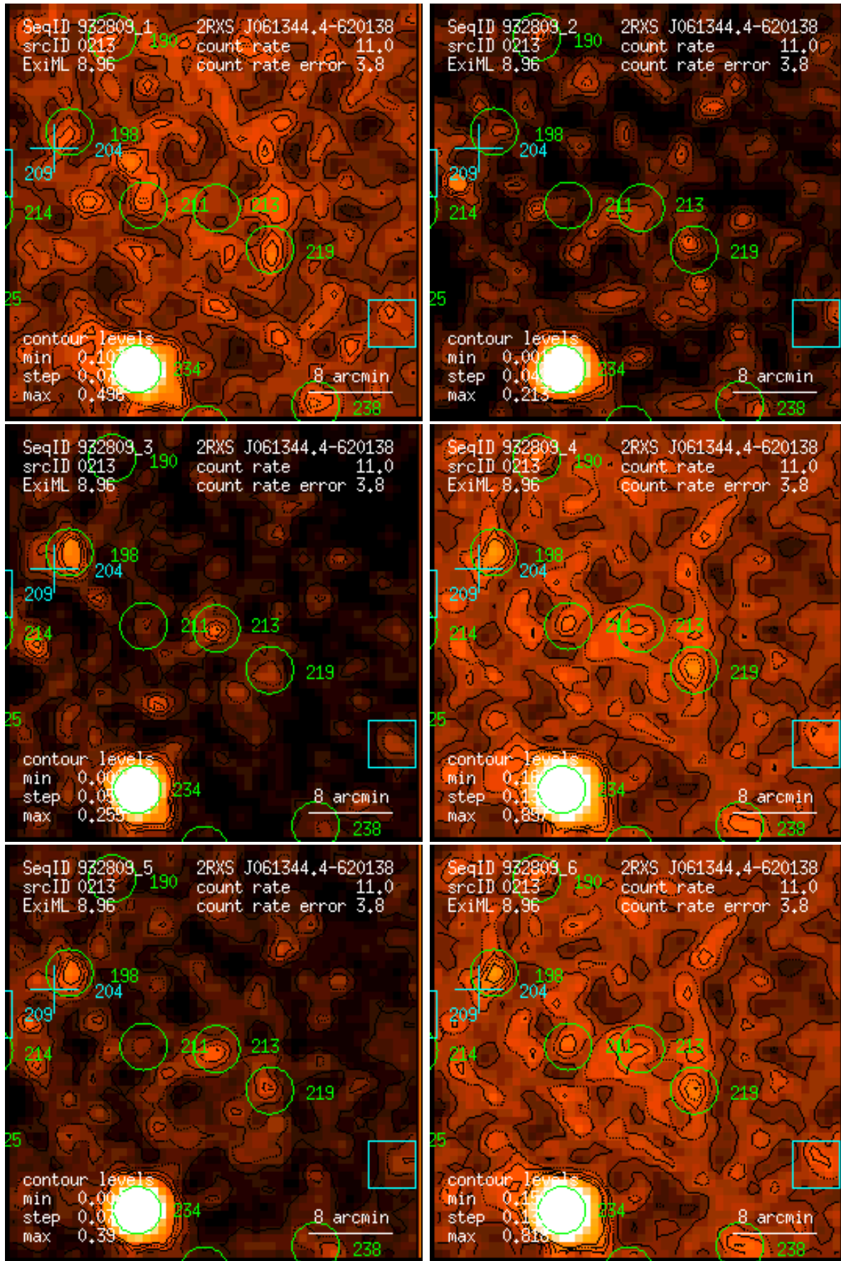
Figure 213: RASS 932809: detection 0213: band rate images, Gaussian filter: (1) PSPC channels 11 – 41, (2) 52 – 90, (3) 91 – 201, (4) 11 – 235, (5) 52 – 201, (6) 11 – 201. Broad band rates in counts/ks. Band rate contour levels in counts/ks/arcmin 2 .
