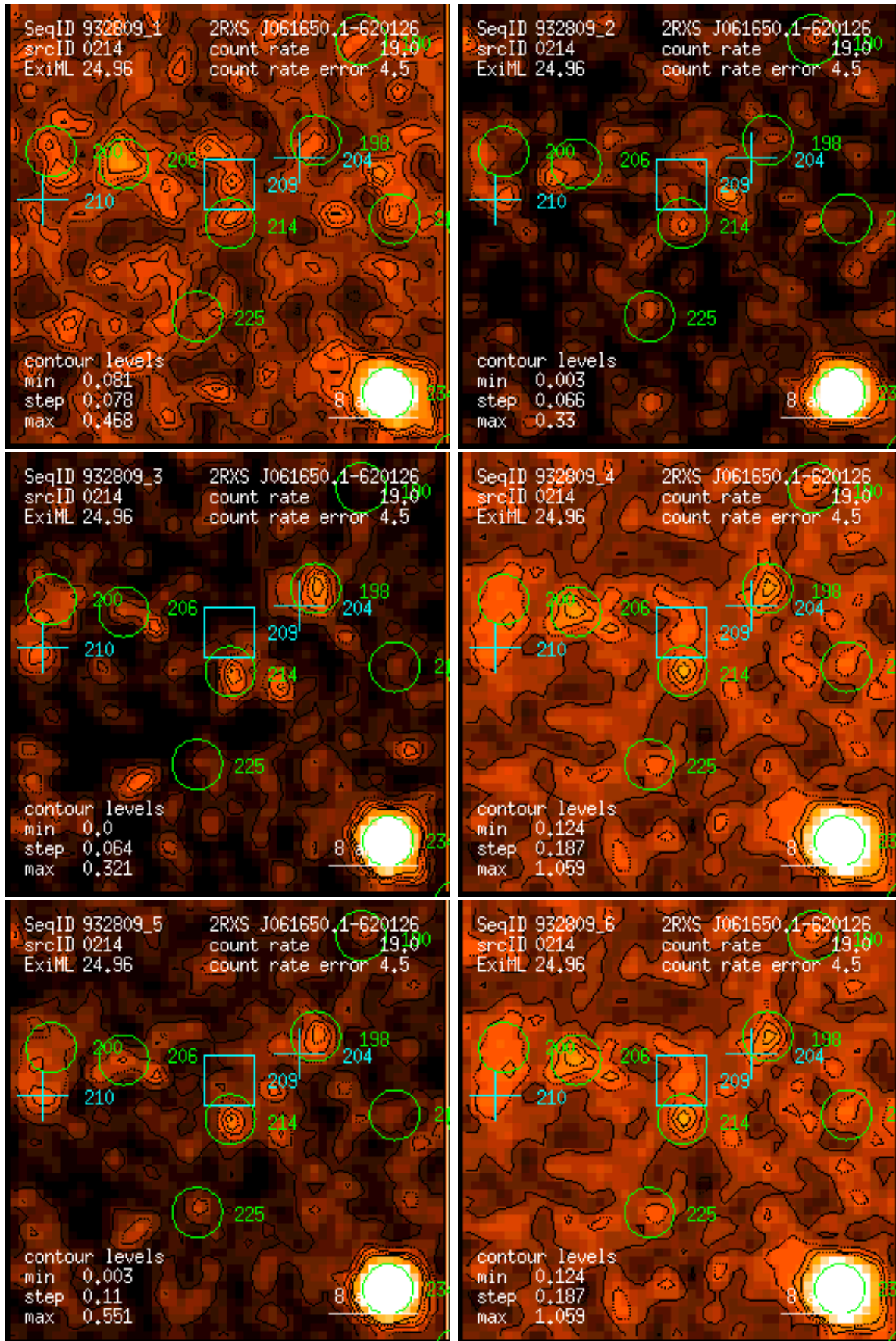
Figure 214: RASS 932809: detection 0214: band rate images, Gaussian filter: (1) PSPC channels 11 – 41, (2) 52 – 90, (3) 91 – 201, (4) 11 – 235, (5) 52 – 201, (6) 11 – 201. Broad band rates in counts/ks. Band rate contour levels in counts/ks/arcmin 2 .
