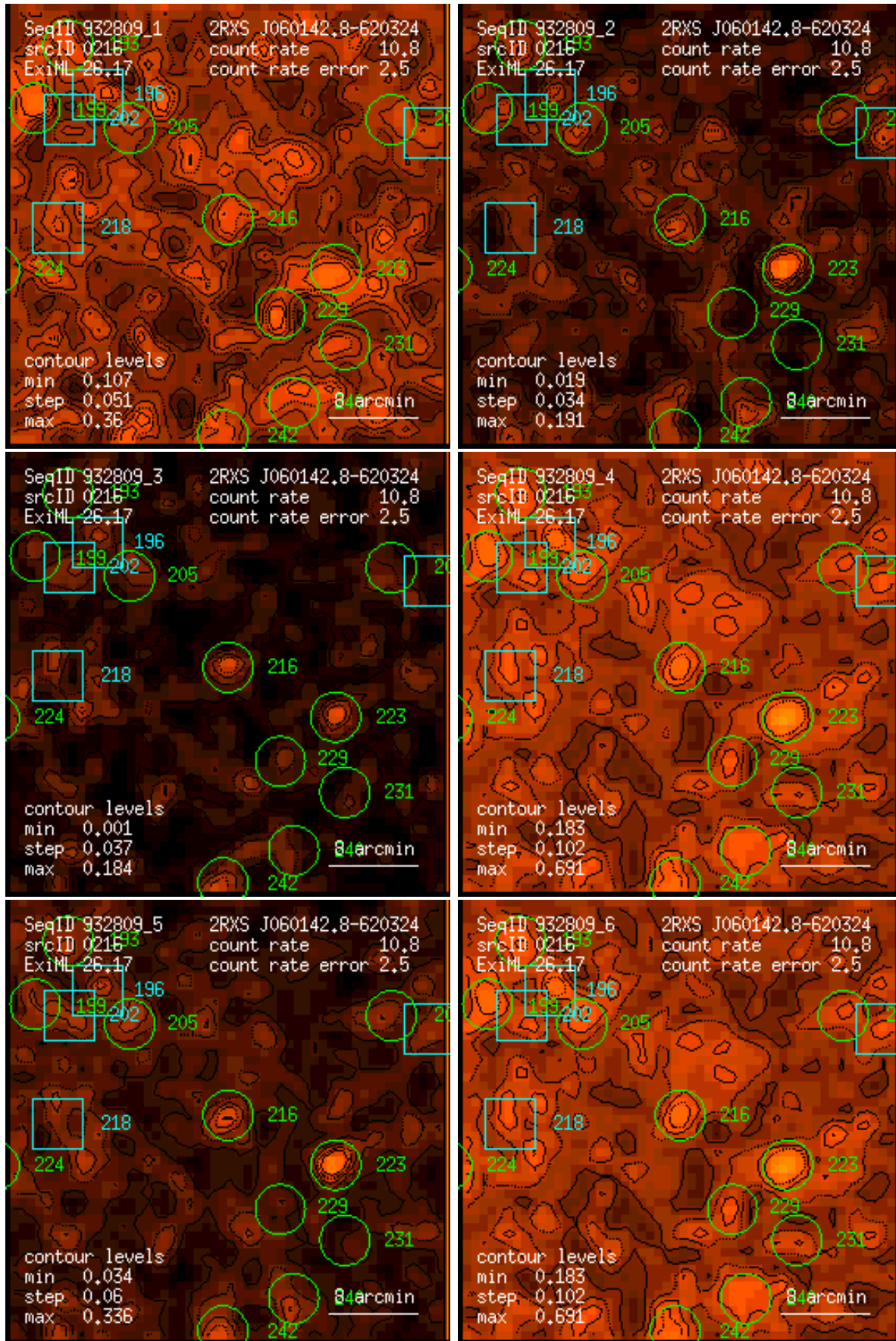
Figure 216: RASS 932809: detection 0216: band rate images, Gaussian filter: (1) PSPC channels 11 – 41, (2) 52 – 90, (3) 91 – 201, (4) 11 – 235, (5) 52 – 201, (6) 11 – 201. Broad band rates in counts/ks. Band rate contour levels in counts/ks/arcmin 2 .
