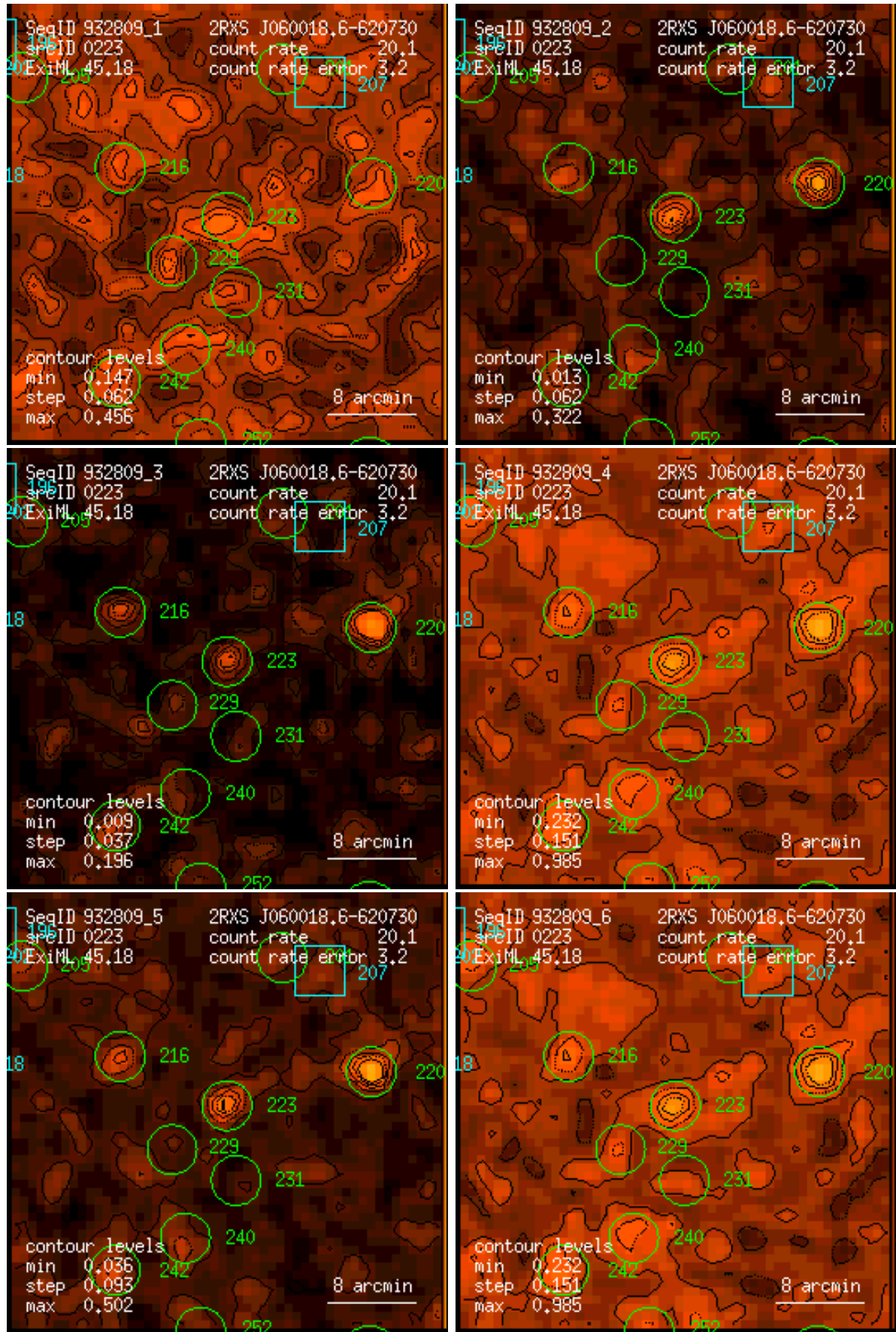
Figure 223: RASS 932809: detection 0223: band rate images, Gaussian filter: (1) PSPC channels 11 – 41, (2) 52 – 90, (3) 91 – 201, (4) 11 – 235, (5) 52 – 201, (6) 11 – 201. Broad band rates in counts/ks. Band rate contour levels in counts/ks/arcmin 2 .
