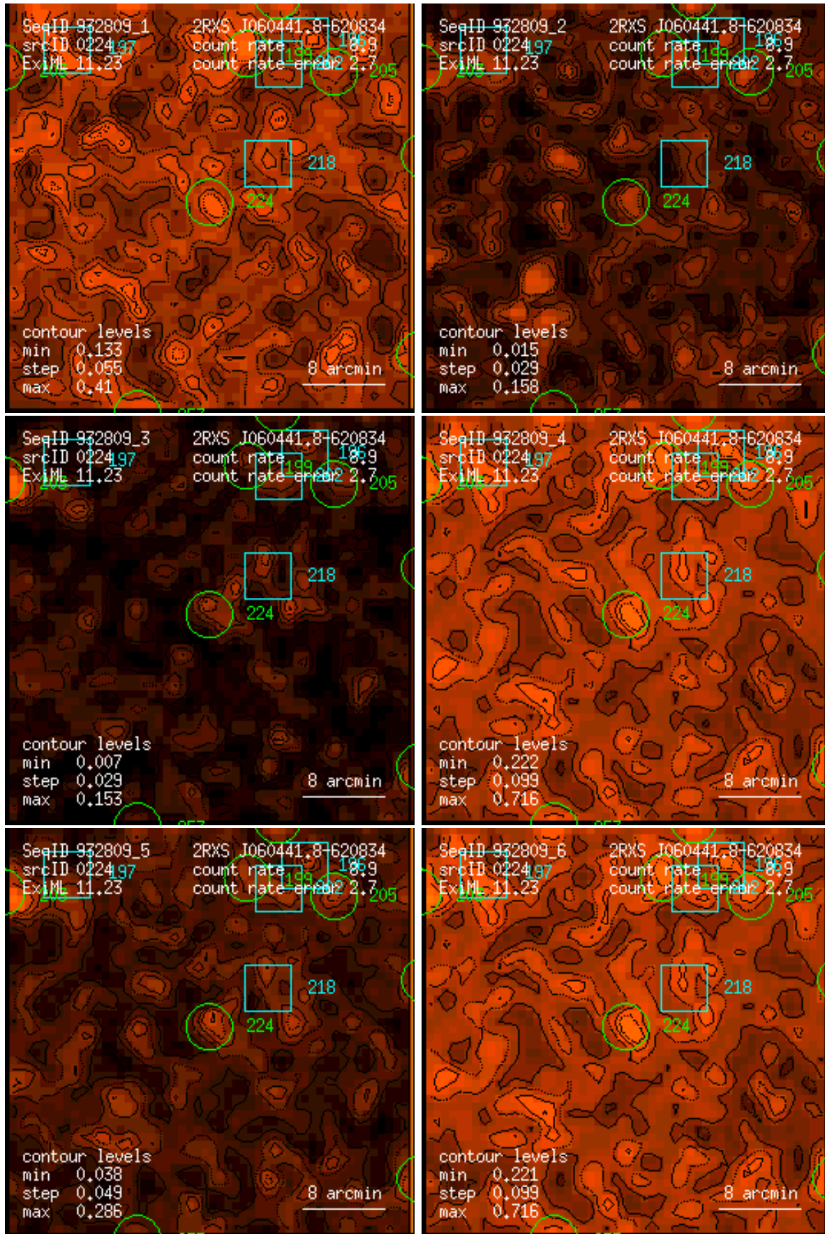
Figure 224: RASS 932809: detection 0224: band rate images, Gaussian filter: (1) PSPC channels 11 – 41, (2) 52 – 90, (3) 91 – 201, (4) 11 – 235, (5) 52 – 201, (6) 11 – 201. Broad band rates in counts/ks. Band rate contour levels in counts/ks/arcmin 2 .
