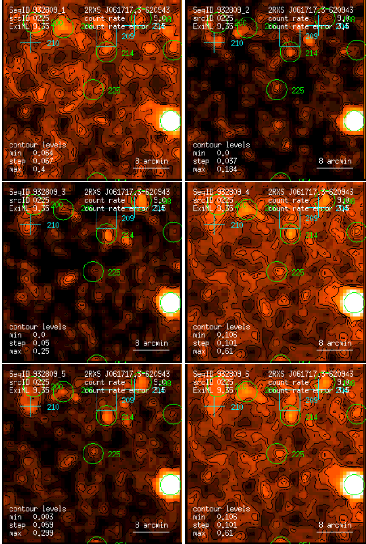
Figure 225: RASS 932809: detection 0225: band rate images, Gaussian filter: (1) PSPC channels 11 – 41, (2) 52 – 90, (3) 91 – 201, (4) 11 – 235, (5) 52 – 201, (6) 11 – 201. Broad band rates in counts/ks. Band rate contour levels in counts/ks/arcmin 2 .
